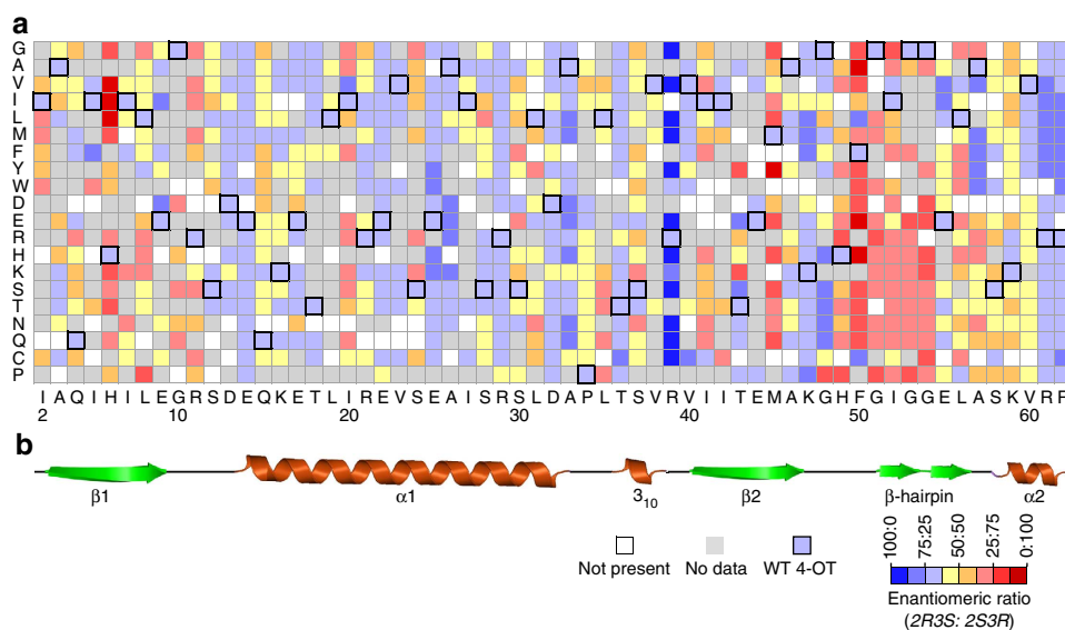
Figure 5 | Mutability landscape of 4-OT for enantioselectivity in the Michael-type addition of 4 to 5a . (a) The horizontal axis of the data matrix depicts the wild-type sequence of 4-OT and the vertical axis depicts the 20 possible amino acid residues. The wild-type amino acid residue at each position is indicated by bold squares and white boxes represent mutants that are not present in the collection. The colour indicates the e.r. (2R3S:2S3R) of the major syn diastereoisomer of 7 as produced by the 4-OT variants. The e.r. values were determined by HPLC on a chiral stationary phase. Grey boxes represent mutants that did not produce sufficient amounts of 7 to give an adequate ultraviolet signal during HPLC analysis. As expected, these grey boxes mainly coincide with the grey and dark blue boxes in Fig. 3c, which indicate mutants that either did not express or lack significant 'Michaelase' activity. (b) The secondary-structure elements of 4-OT 20 .
