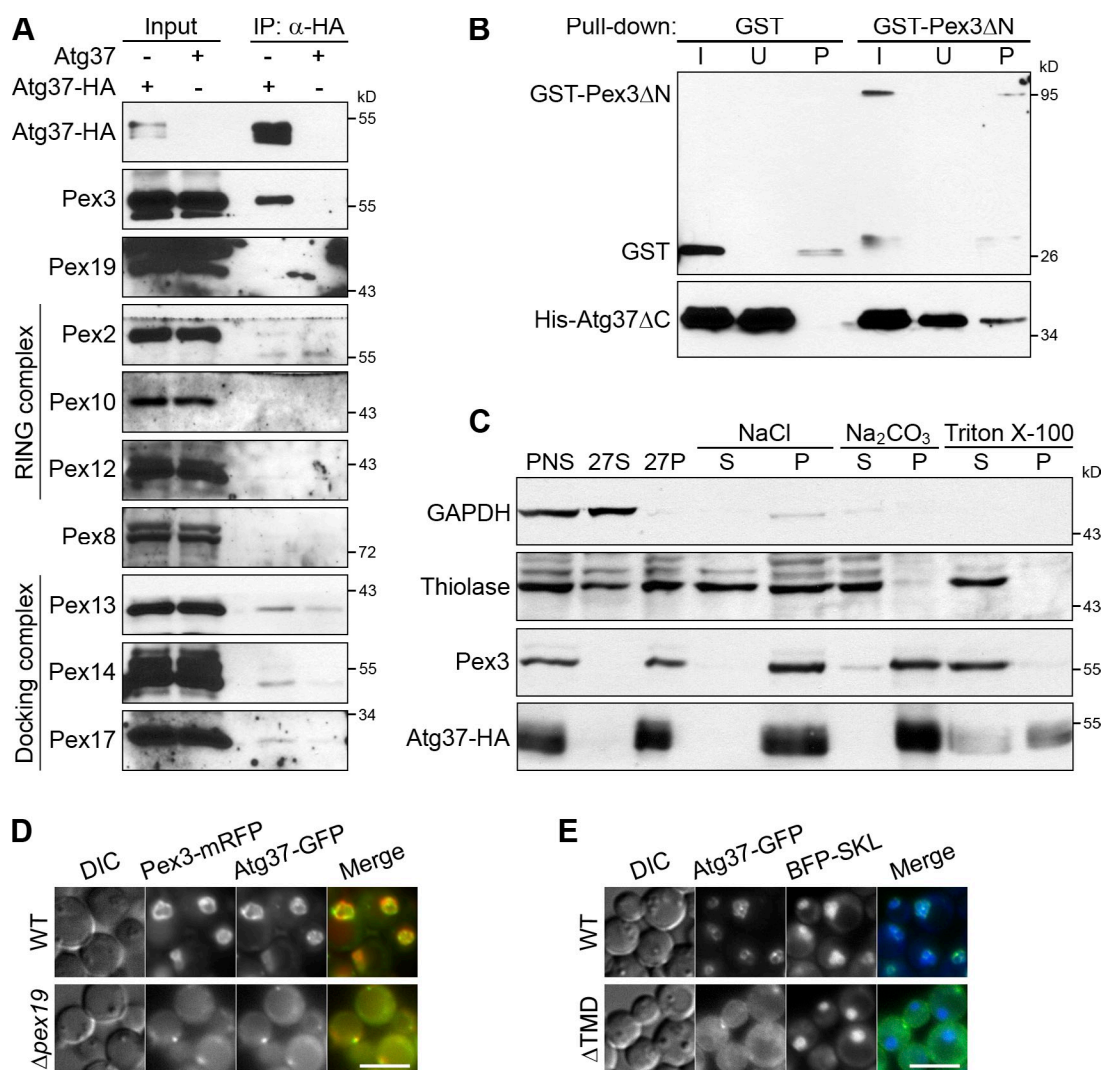
Figure 1. Atg37 is an integral PMP that binds Pex3. (A) Pex3 coimmunoprecipitates with Atg37. IP, immunoprecipitate. Cells were induced in methanol medium for 4 h. (B) Atg37ΔC binds Pex3ΔN in vitro. I, input; U, unbound; P, pull-down. (C) Atg37 is an integral membrane protein. PNS, postnuclear supernatant; 27S, 27,000 g supernatant; 27P, 27,000 g pellet; S, 200,000 g supernatant; P, 200,000 g pellet. (D) Atg37 localizes to the peroxisomal membranes (in WT) or ER-associated peroxisome remnants labeled with Pex3-mRFP (in \Delta pex19 ). DIC, differential interference contrast. Bar, 5 \mu m. (E) The TMD is essential for peroxisomal localization of Atg37. SKL, Ser-Lys-Leu, a peroxisomal targeting signal. Bar, 5 \mu m.
