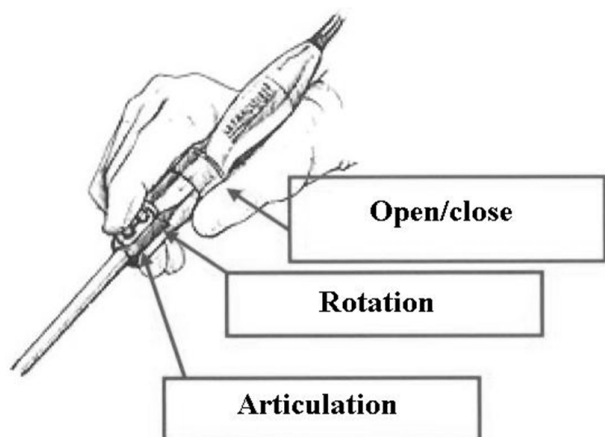
Figure 4 Proposal for an electronic handle for the Roticulator Endo Mini-Shears™.
