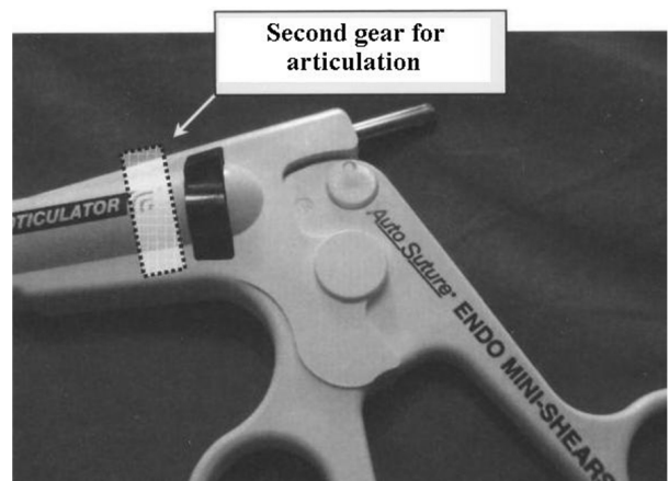
Figure 3 Proposed position for the second gear on the Roticulator Endo Mini-Shears™.
