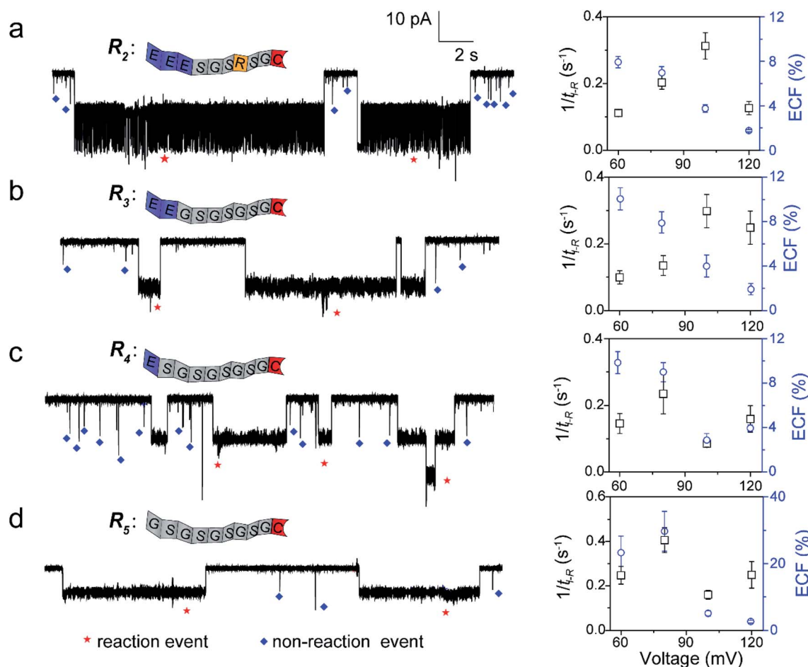
Fig. 3 The single-molecule reaction of \mathbf{R}_2 (a), \mathbf{R}_3 (b), \mathbf{R}_4 (c), and \mathbf{R}_5 (d) with a K238C AeL nanopore. Left: the ionic current trace at +60 mV. The red and blue symbols represent the reaction events, and non-reaction events, respectively. Right: voltage dependent of the reaction rate ( f_{\text{PR}} = 1/t_{\text{R}} ) and ECF. The current fluctuation of the reaction events may be attributed to the conformational changes of the peptide or the possible intermediates. All data were acquired at 20.0 \pm 2.0 °C in 1.0 M KCl, 10.0 mM Tris, and 1.0 mM EDTA solution buffered at pH 8.0 in the presence of 50.0 \mu\text{M} reactant. The short bumping events have been excluded.
