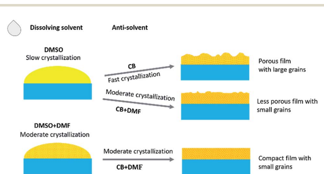
Fig. 1 Schematic illustration for the effects of the solvents on the crystallization processes and the resultant morphology of the quasi-2D perovskite films.
