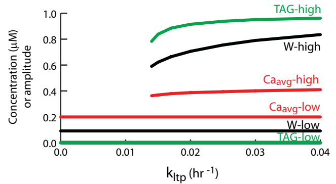
Figure 4. A bifurcation diagram illustrates bistability of synaptic weight. The bifurcation parameter k_{ltp} is the rate constant for increases in W during L-LTP. As k_{ltp} increases past 0.014, a steady state of high W appears. In this state, the time average of synaptic [Ca^{2+}] is elevated (running average taken over 10 min of Ca^{2+} transients). Consequently the tag for L-LTP is set ( TAG is near 1.0), allowing for continual reinforcement of L-LTP. Synaptic [Ca^{2+}] is vertically scaled by 4.0. Parameters other than k_{ltp} are at their standard values (Table 1). doi:10.1371/journal.pone.0000445.g004
