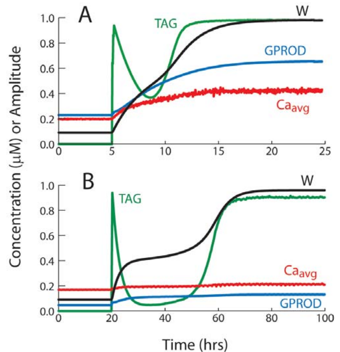
Figure 5. Time courses of W , GPROD, TAG, and time-averaged synaptic Ca^{2+} following 3 tetani to the single synapse of Fig. 4. Tetanus parameters are as in Fig. 2. Initially, W is in the low steady state of Fig. 4. The tetani elevate TAG, GPROD, and W . (A) With continuous background synaptic activity, TAG, GPROD, and W converge to the high steady state of Fig. 4. k_{ltp} = 0.4 \text{ hr}^{-1} , well to the right of the range in Fig. 4, so the high state of W is close to 1. Synaptic [Ca^{2+}] is vertically scaled by 4.0 and GPROD is scaled by 0.5. Other parameters are as in Figure 4. (B) Tetani also induce a transition to the high steady state with episodic, rather than continuous, background synaptic activity. Periods (15 sec) of brief Ca_{syn} and Ca_{nuc} elevations at theta-rhythm frequency are separated by intervals (45 sec) with no activity. All other parameters are as in (A) except k_{ltp} = 1.0 \text{ hr}^{-1} . doi:10.1371/journal.pone.0000445.g005
