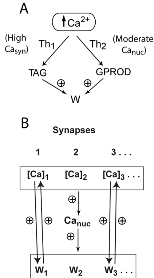
Figure 1. Schematic of the model for L-LTP induction. Electrical stimuli (tetanus or theta-burst) elevate synaptic and nuclear Ca^{2+} . Steep sigmoidal functions of synaptic Ca^{2+} and nuclear Ca^{2+} transduce Ca^{2+} elevations into activation of synaptic tagging (elevation of the variable TAG) and activation of gene expression (elevation of GPROD). These sigmoidal functions are denoted Th_1 and Th_2 . Equations are given in Methods. High synaptic Ca^{2+} elevations are required to set the tag for L-LTP. L-LTP is simulated by increase of a synaptic weight W at a rate proportional to the product of TAG and GPROD. (B) Model of a group of synapses converging on a single postsynaptic neuron. At each synapse, ongoing activity is modeled with brief Ca^{2+} transients at theta frequency (see Methods for details). Strengthening of any of the weights W_1 \dots W_N increases the amplitude of Ca^{2+} transients at that synapse and the level of nuclear Ca^{2+} . In turn, increased synaptic Ca^{2+} synergizes with increased nuclear Ca^{2+} to strengthen the corresponding synaptic weight. doi:10.1371/journal.pone.0000445.g001
