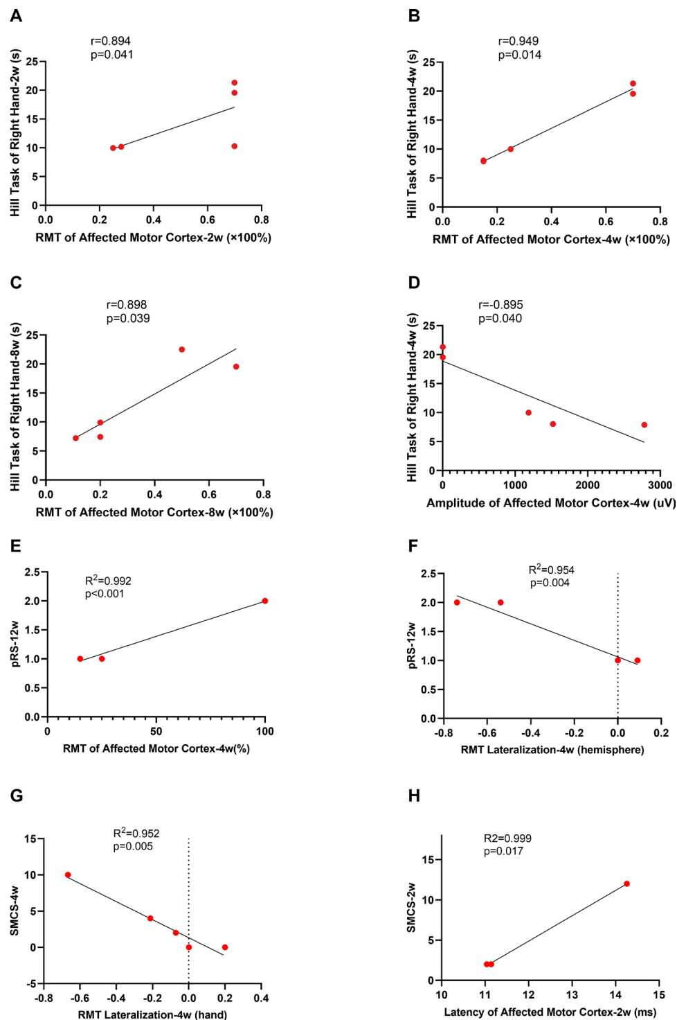
Figure 8 Correlation analysis.
