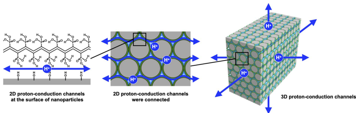
Scheme 1 Schematic model of proton-conductive core-shell nanoparticle-filled PEM.
