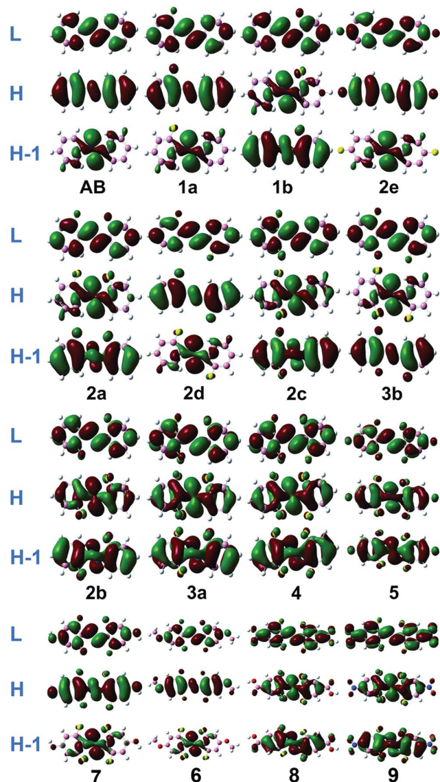
Fig. 3 Molecular orbital profiles of the E isomers of azobenzene compounds. Notes: L, H and H-1 represent LUMO, HOMO and HOMO-1 respectively.
