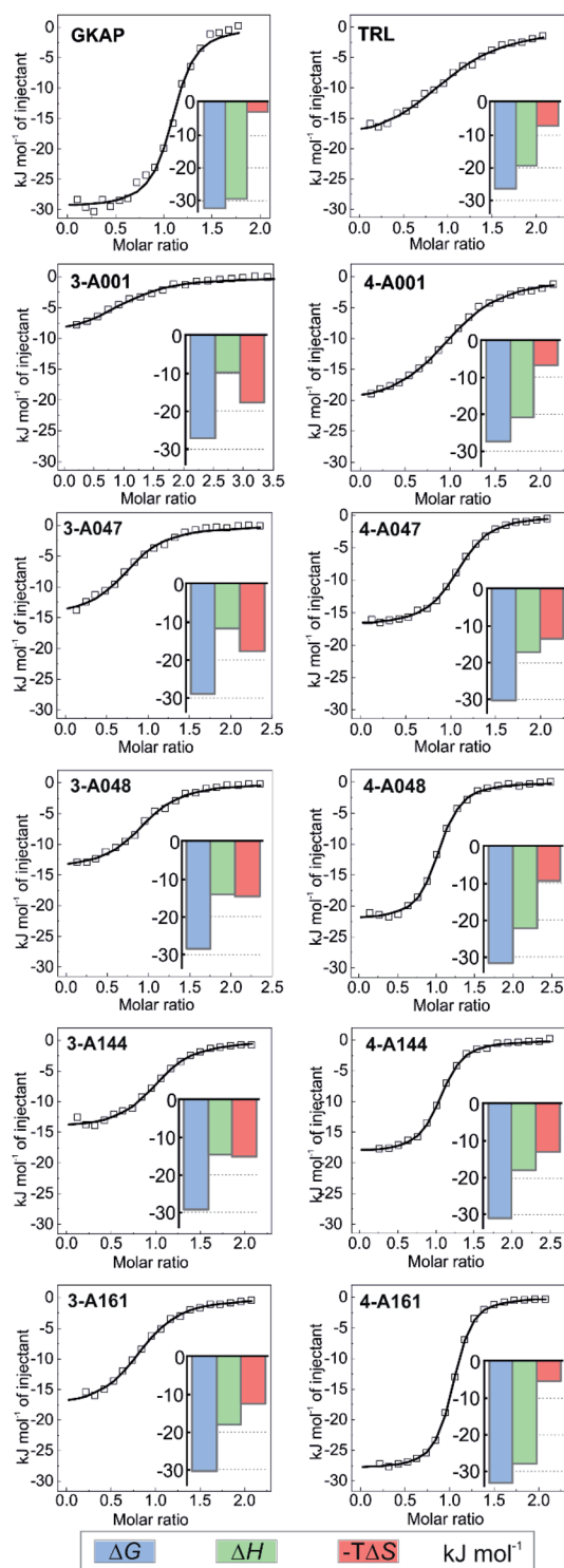
Fig. 4 Hit validation by ITC. Fitted thermograms and thermodynamic signatures for the tested peptides and hydrazones. ITC data were acquired in 25 mM Tris, pH 7.5 buffer containing 150 mM NaCl at 25 °C by injecting 0.75–1 mM peptide or hydrazone solution into 75–150 \mu M protein in the cell. For individual raw ITC data and fitted thermograms see Fig. S14.†
