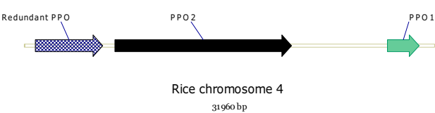
Figure 6 Schematic representation of PPO gene cluster in rice taken from rice chromosome 4 [GenBank: AP008210.1 31754771–31786730]. PPO1: [GenBank: AK108237.1 ] (DNA), [PDB: CAE03510.2 ] (amino acid); PPO2: [PDB: CAH66801.1 ] (amino acid).
