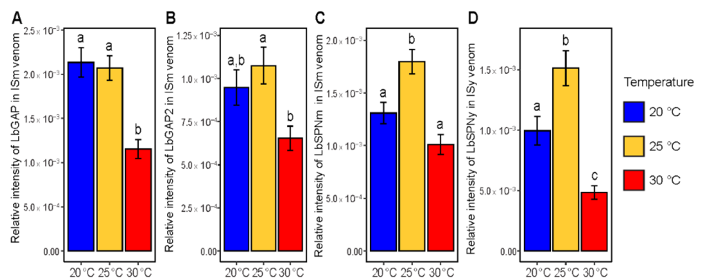
Figure 6. Impact of temperature during parasitoid nymphal development on the amount of specific proteins in the venom. Relative amount of LbGAP (A), LbGAP2 (B) and LbSPNm (C) in L. boulandi ISm venom and of LbSPNy in L. boulandi ISy venom (D). Different letters indicate a significant difference between temperatures. Bars indicate standard errors.
