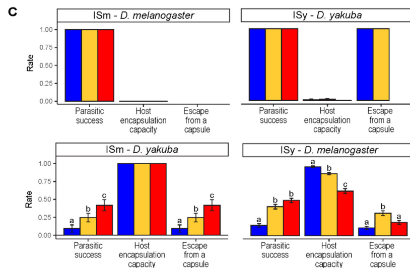
Figure 2. Impact of temperature during parasitism on the outcome of host–parasitoid interaction. (A) Possible outcomes in parasitized Drosophila larvae 48–72 h after parasitism and details of analyzed parameters: parasitic success, host encapsulation capacity, parasitoid ability to inhibit encapsulation and parasitoid capacity to escape from a capsule. (B) Parasitism rates for the four host–parasitoid interactions as a function of temperature. (C) Rate of (i) parasitic success, (ii) host encapsulation capacity or (iii) parasitoid capacity to escape from a capsule, depending on the temperature. Within each host–parasitoid interaction, different letters indicate a significant difference between temperatures for a given parameter. Bars indicate standard errors (see Supplementary Tables S1 and S2 for sample sizes and statistical outputs).
