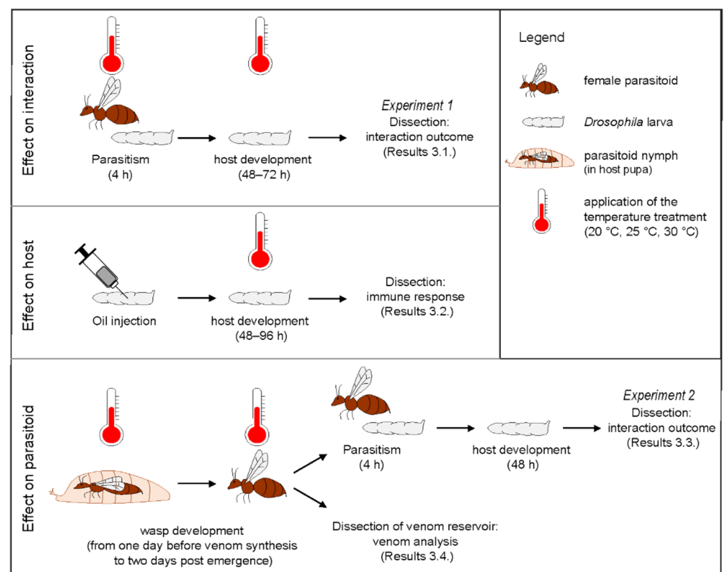
Figure 1. Schematic illustration of the experimental designs. A thermometer indicates where different temperatures ( 20\text{ }^{\circ}\text{C} , 25\text{ }^{\circ}\text{C} or 30\text{ }^{\circ}\text{C} ) were applied, while the absence of a thermometer means that the step was performed at 25\text{ }^{\circ}\text{C} .
