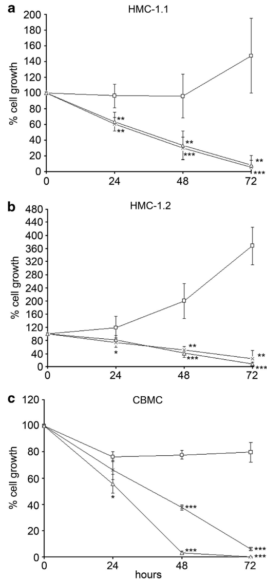
Figure 1 MG132 inhibits cell growth of human mast cells with activated Kit. Kinetic curves of MG132-treated (a) HMC-1.1 (V560G mutation), (b) HMC-1.2 (V560G and D816V mutations) and (c) CBMCs (activated with SCF), where \square indicates control cells, \times 1 \mu M MG132 and \Delta 10 \mu M MG132-treated cells. Viable cells were quantified by trypan blue exclusion criteria. Mean \pm S.D., n=3 . * P<0.05 , ** P<0.01 and *** P<0.001
