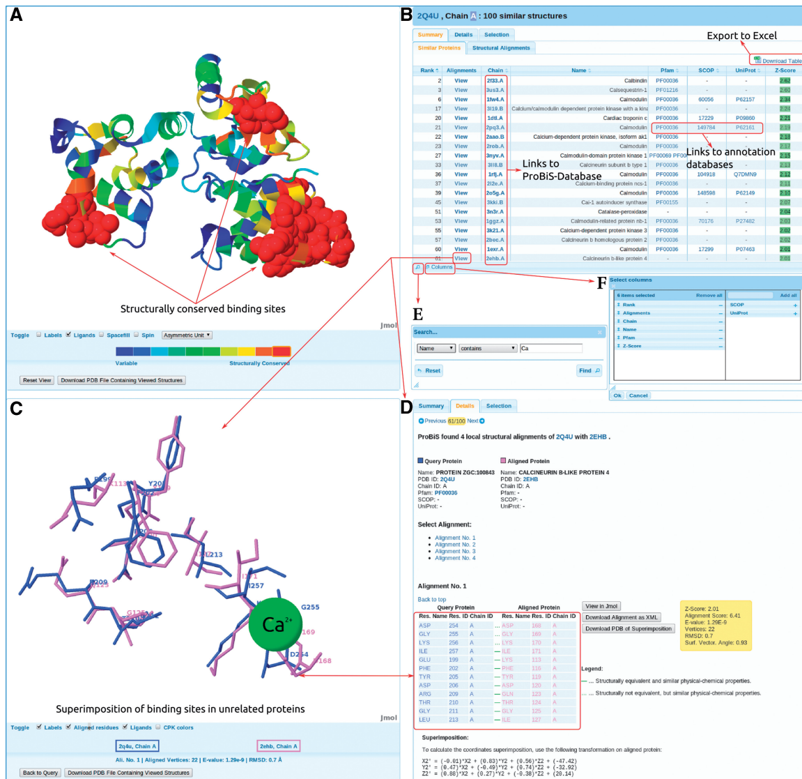
Figure 3. ProBiS output page for query protein (PDB/Chain ID: 2q4u.A) of unknown function. (A) Structurally conserved binding sites. (B) An interactive table of similar proteins, filtered to show only calcium binding proteins. (C) Local structural superimposition of the blue query (2q4u.A) and the violet similar protein (2ehb.A) that contains a co-crystallized Ca^{2+} ion shown as green sphere. (D) The alignments presented as tables of residue-residue correspondences. (E) Integrated search tool. (F) Columns reordering tool.
