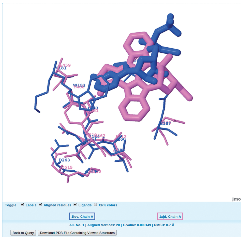
Figure 4. Superimposition of similar binding sites in Ddl (1iov.A; blue) and PKC (1xjd.A; violet). The superimposed residues from Ddl and protein kinase C are shown as thin wireframe models. The co-crystallized ligands, ADP (blue) and staurosporine (violet), are shown as thick wireframe models.
