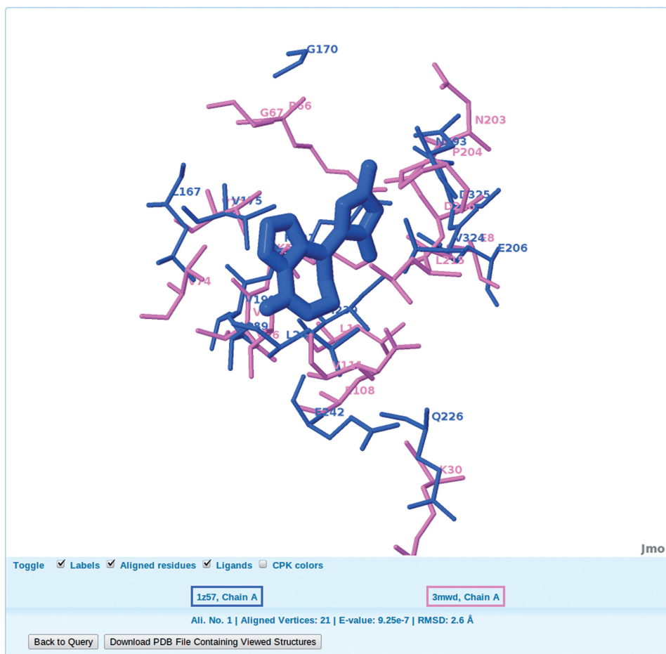
Figure 5. Superimposition of similar binding sites in dual-specificity kinase (1z57.A; blue) and ATP-citrate synthase (3mwd.A; violet). The superimposed residues are thin wireframe models. The inhibitor debromohymenialdisine is colored blue and is a thick wireframe model.
