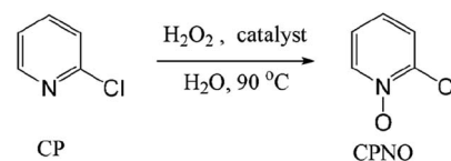
Scheme 1 Catalytic oxidation of CP to CPNO using H 2 O 2 and an anhydride catalyst.
