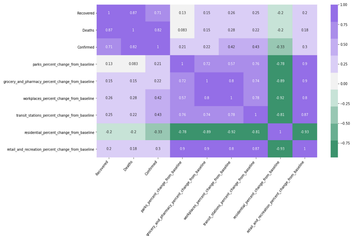
Fig. 4. Pearson correlation of weekly mean confirmed, recovered, death cases and weekly mean human activities of all countries with off set of -2.
