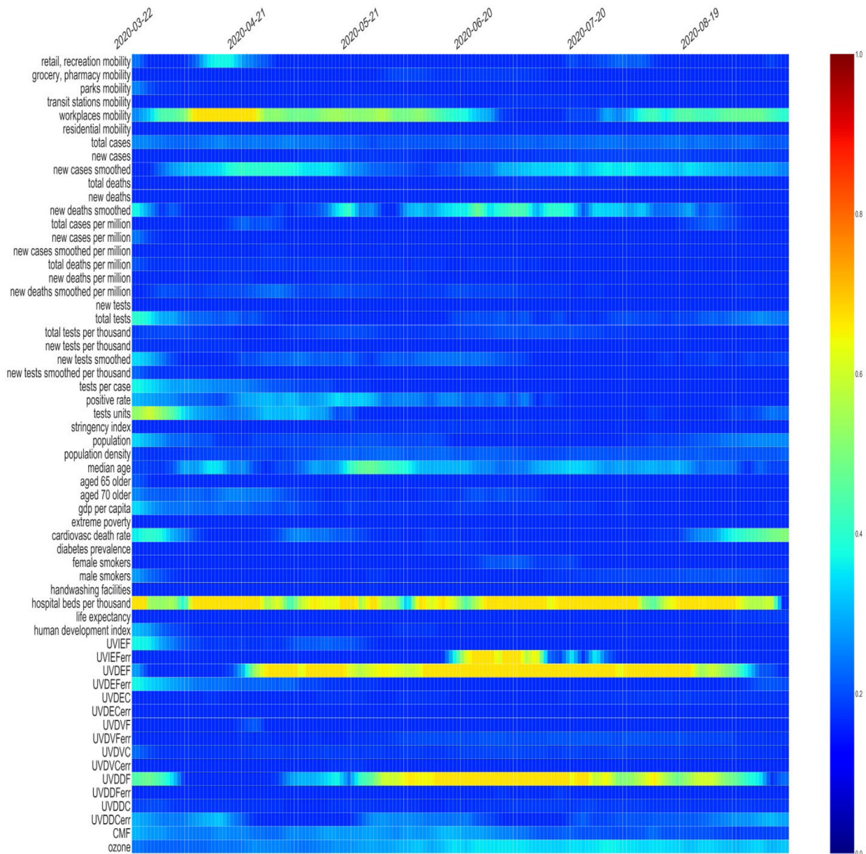
Fig. 12. Time and feature attention corresponding to a prediction for new daily COVID-19 cases in Sweden.
