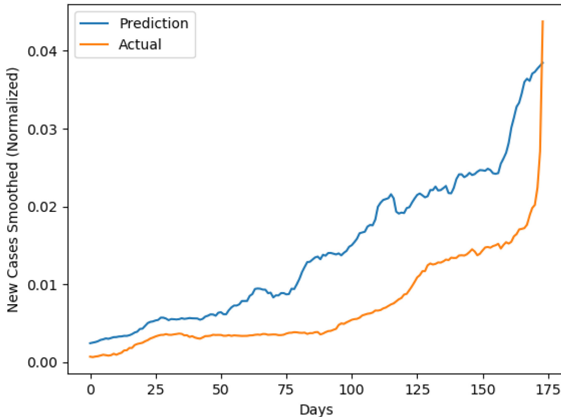
Fig. 9. Actual and reconstruction of Sweden.
