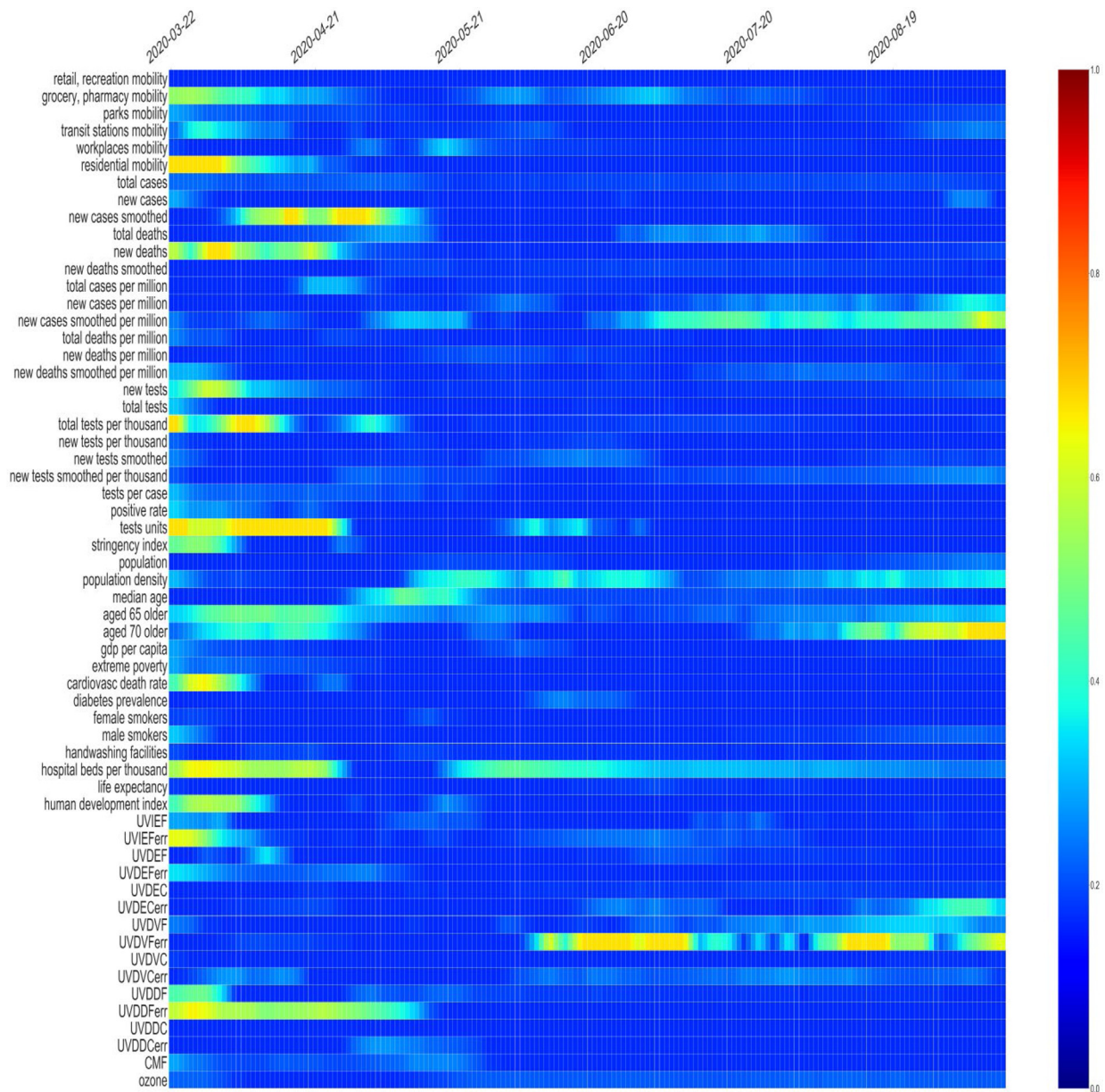
Fig. 14. feature attention corresponding to a prediction for new daily COVID-19 cases in Norway.
