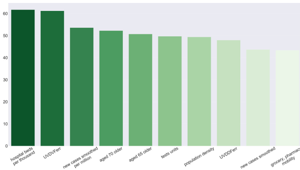
Fig. 15. Temporal aggregation of attribution in Italy (x-axis is variables and y-axis is aggregation score).
