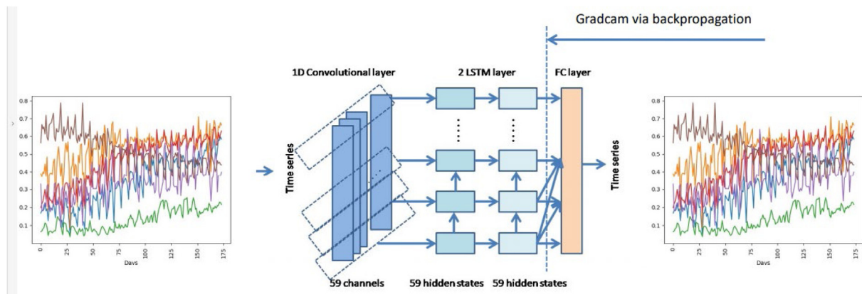
Fig. 5. Convolution-LSTM architecture and its visual attribution via Gradcam.
