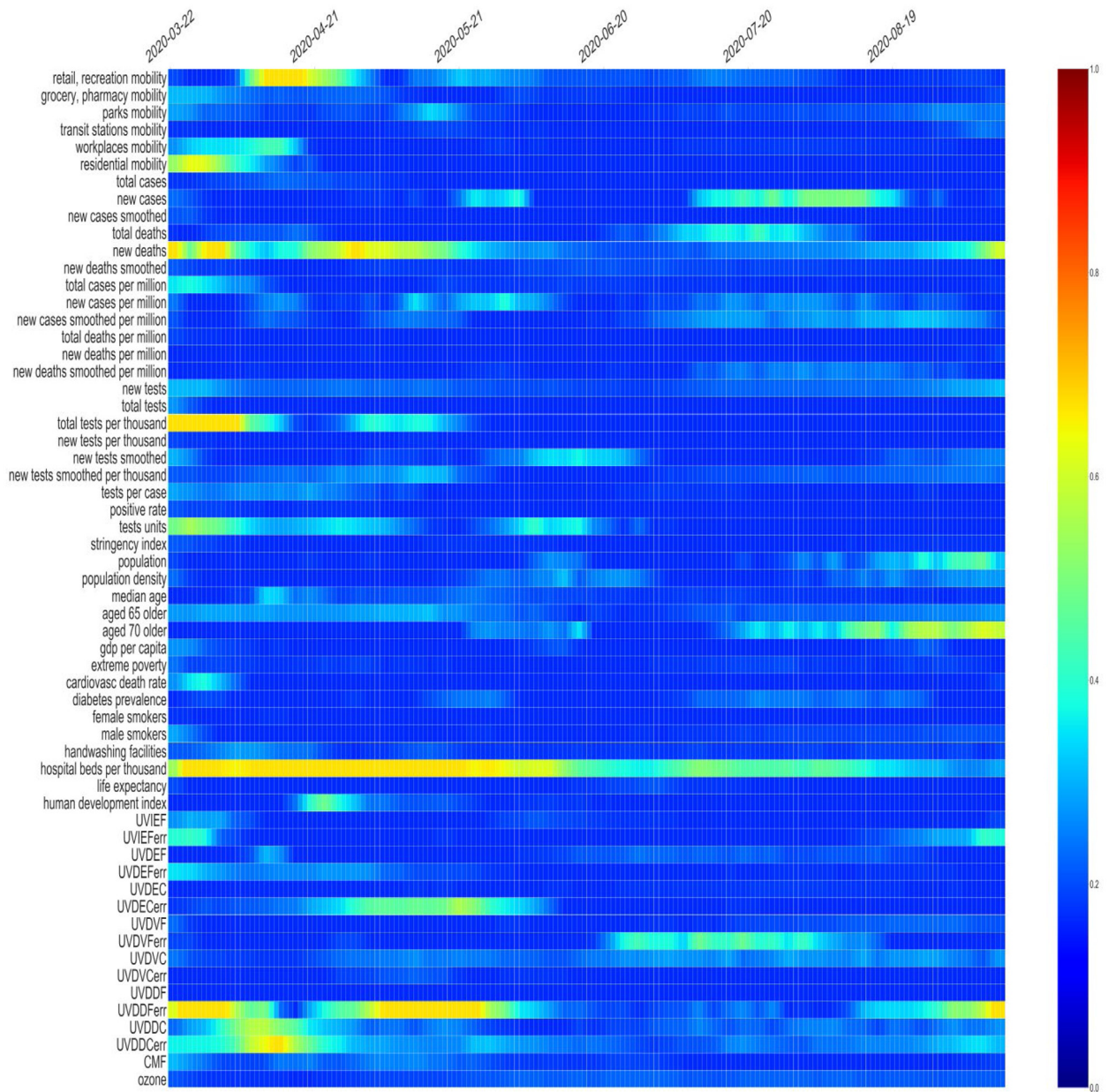
Fig. 10. Time and feature attention corresponding to a prediction for new daily COVID-19 cases in Italy.
