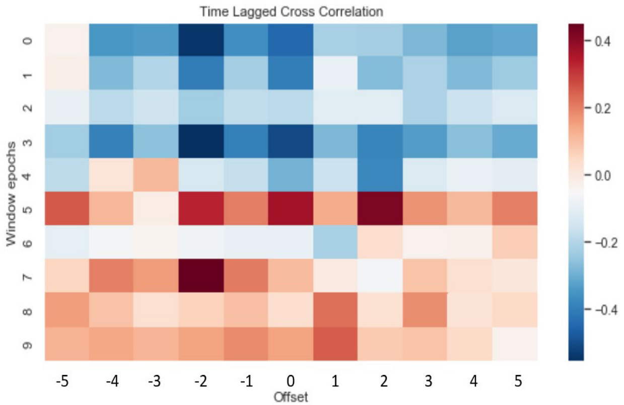
Fig. 3. Time lagged cross-correlation between weekly mean confirmed cases and human activities in Jakarta region.
