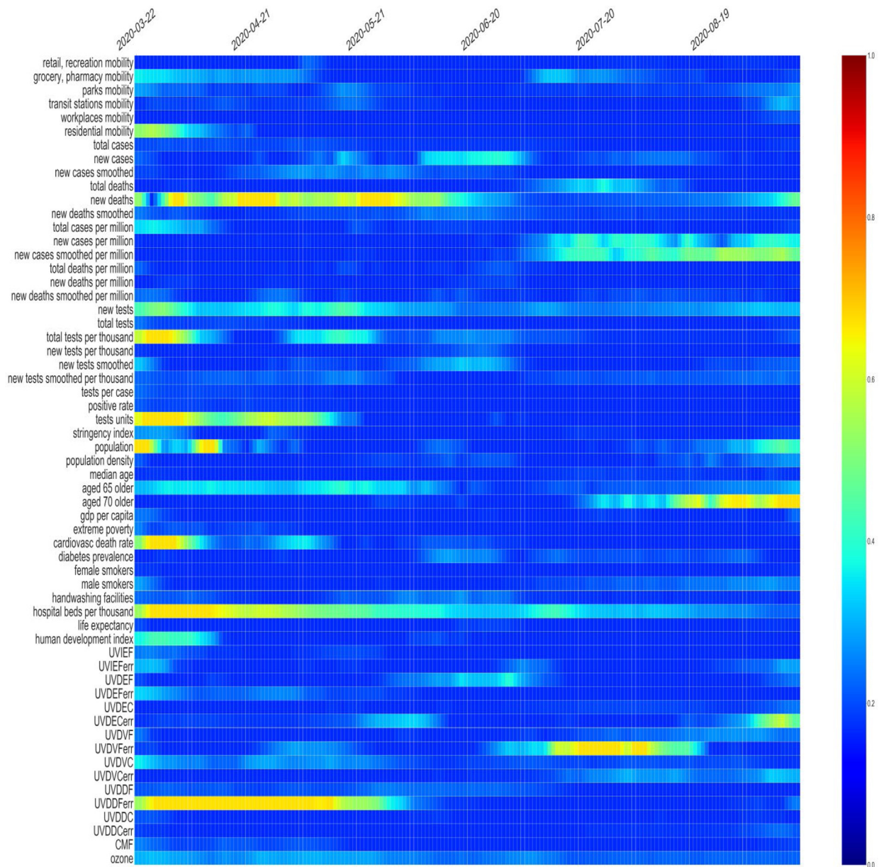
Fig. 16. Time and feature attention corresponding to a prediction for new daily COVID-19 cases in Indonesia.
