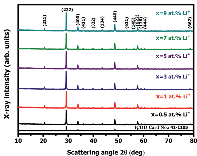
Fig. 1 X-ray diffraction (XRD) pattern of \text{Y}_2\text{O}_3:4 \text{ at\% Eu}^{3+} , x\text{Li}^+ ( x = 0.5, 1, 3, 5, 7, 9 \text{ at\%} ) nanophosphors.
