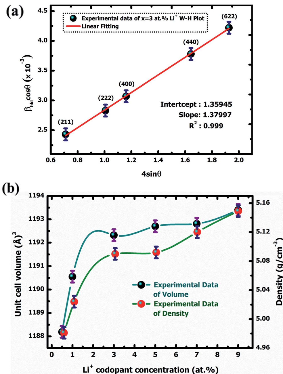
Fig. 2 W–H plot of Y_2O_3:4 \text{ at\% } Eu^{3+} , xLi^+ (a) x = 3 \text{ at\%} nanophosphor (b) variation of unit cell volume and density with Li^+ codoping concentration.
