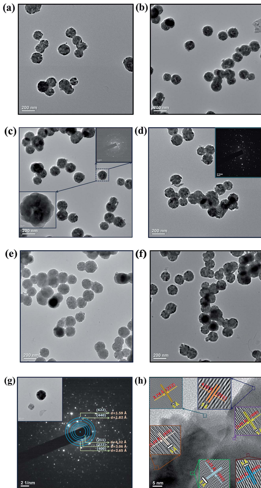
Fig. 6 HR-TEM Images of \text{Y}_2\text{O}_3:4 \text{ at}\% \text{ Eu}^{3+}, x\text{Li}^+ (a) x = 0.5 at%, (b) x = 1 at%, (c) x = 3 at%, (d) x = 5 at%, (e) x = 7 at%, (f) x = 9 at% nanophosphors. (g) The magnified HR-TEM image and SAED pattern analysis of x = 9 at% prepared crystalline sample. (h) Lattice fringes of x = 9 at% samples corresponds to cubic yttrium(III) oxide ( \text{Y}_2\text{O}_3 ).
