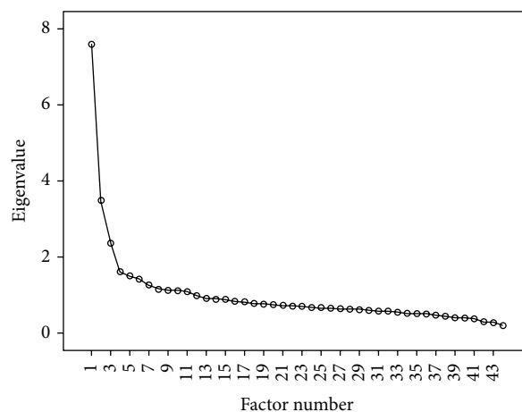
FIGURE 1: Scree plot.
