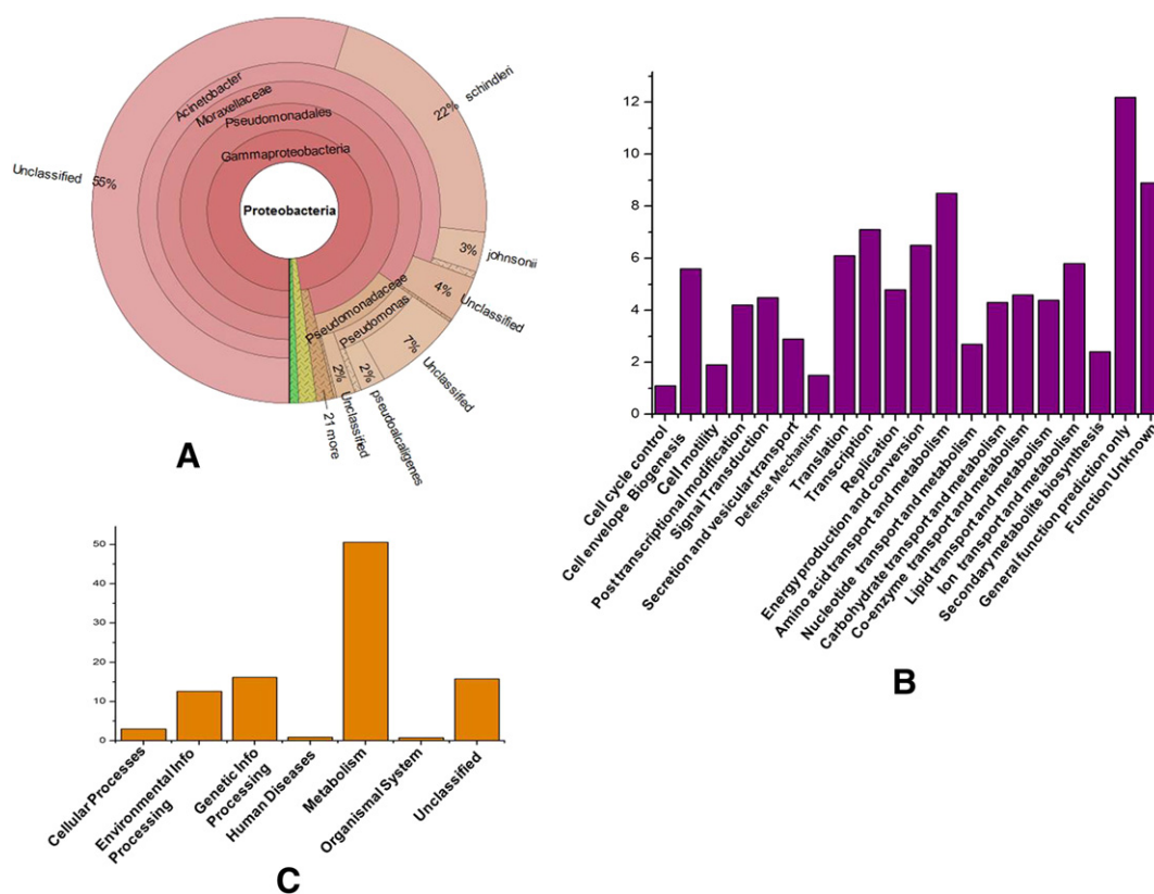
Fig. 2. Abundance and functional predictions of bacterial diversity of Aguas Calientes hot spring (Peru). A: Summary of the phylum Proteobacteria detected in AC in a multilevel chart (Krona); B: COGs metagenome functional predictions of OTUs; and C: KEGG metagenome functional predictions of OTUs using PICRUST tool.
