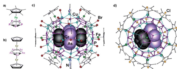
Fig. 1 (a) Building block [Cp*Fe( \eta^5 -P 5 )] (b) template [(CpCr) 2 ( \mu , \eta^{5:5} -As 5 )] ( 1 ); (c) inclusion of 1 into the 90-vertex sphere A; (d) inclusion of 1 into the 16VE fragment [CpCr( \eta^5 -As 5 )] generated from 1 into the 80-vertex sphere B.
