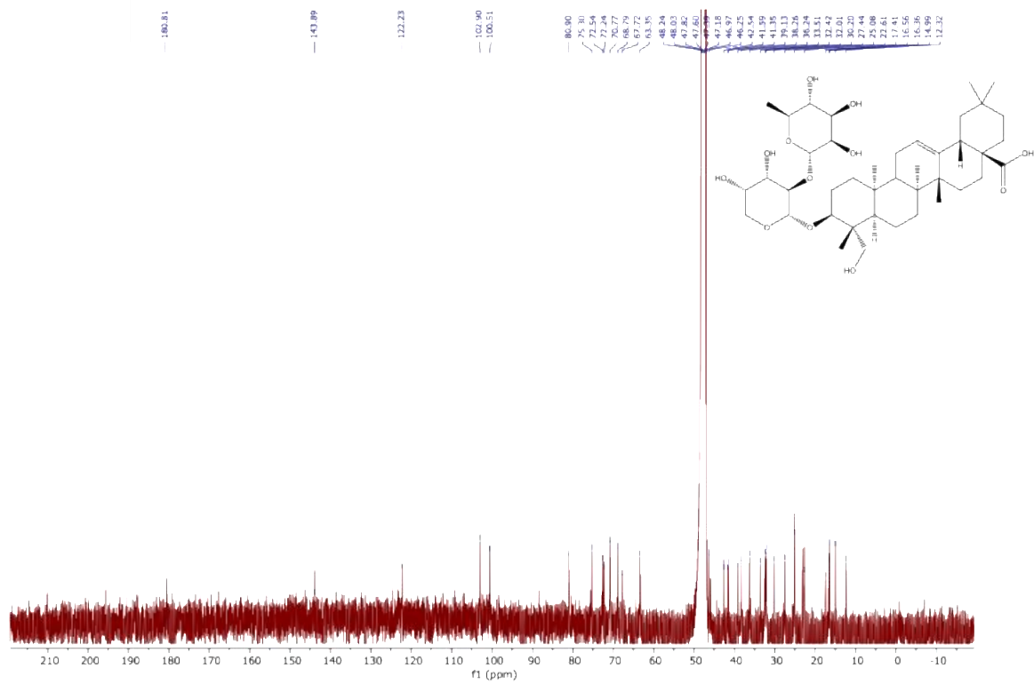
Fig. S2. ^{13}\text{C} NMR of \alpha -hederin.
