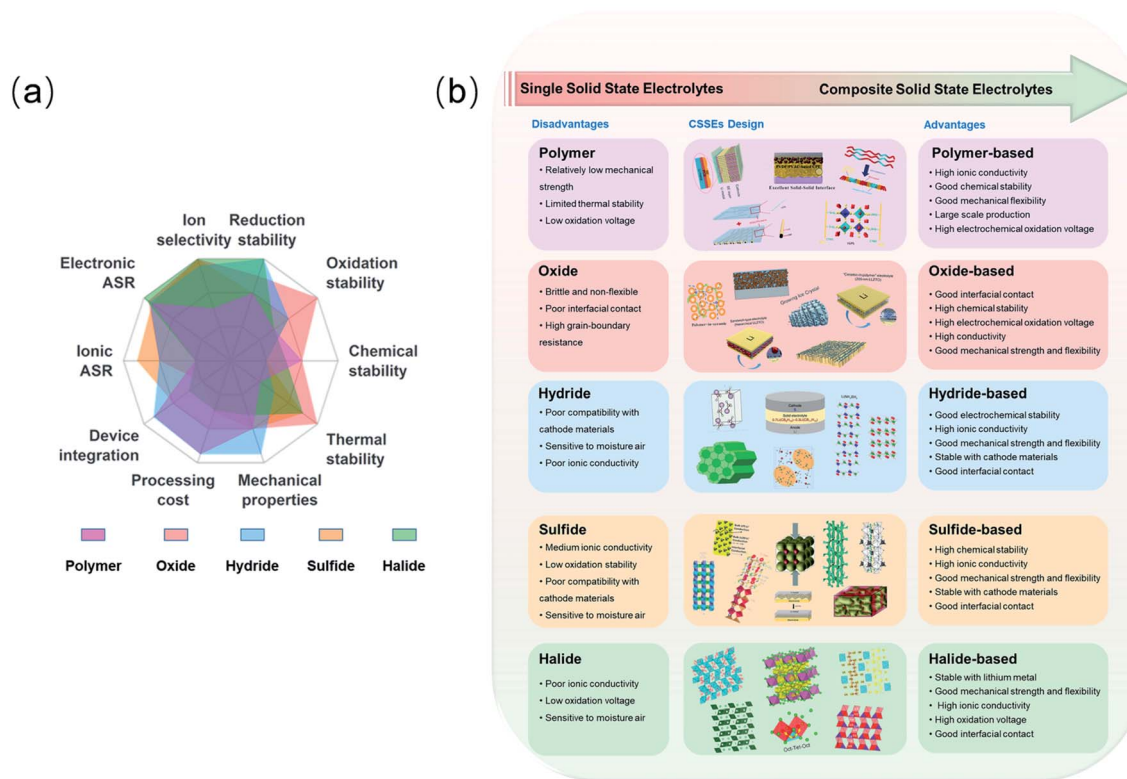
Fig. 1 (a) The superposed radar plot of different types of SSEs and requirements for SSEs. ASR, area-specific resistance. Reproduced from ref. 11 with permission from Springer Nature, copyright 2017. (b) Design of CSSEs from single type SSEs and corresponding physicochemical characteristics.
