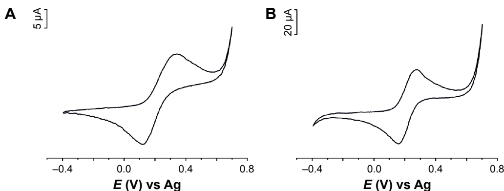
Figure 3 The voltammetric signals of CSPE (A) and GPH-CSPE (B) immersed in 10^{-3} mol \times L ^{-1} K _4 [Fe(CN) _6 ] and 0.2 M KCl at 0.1 V s ^{-1} . Abbreviations: GPH-CSPE, graphene-carbon screen-printed electrode; CSPE, carbon screen-printed electrode.
