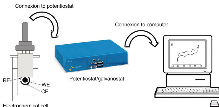
Figure 2 Experimental setup of the electrochemical measurements: electrochemical cell, potentiostat/galvanostat and personal computer. Abbreviations: RE, reference electrode; WE, working electrode; CE, counter electrode.
