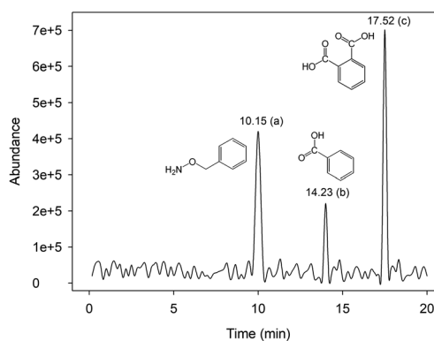
Fig. 7 GC chromatograph of the derivatization products with the Fenton-like system [ \text{pH} = 4.0 , [\text{Fe}^0] = 9 mM, [\text{H}_2\text{O}_2] = 8 mM, [\text{RhB}] = 0.1 mM, and T = 25^\circ\text{C} ].
