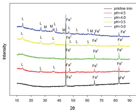
Fig. 5 XRD patterns for different pH levels in the removal of RhB by the Fenton-like system [ [\text{Fe}^0] = 9 mM, [\text{H}_2\text{O}_2] = 8 mM, [\text{RhB}] = 0.1 mM, and T = 25^\circ\text{C} ].
