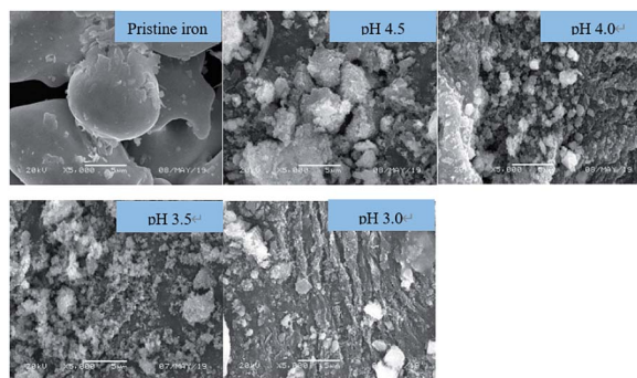
Fig. 6 SEM images of ZVI samples after Fenton-like reaction at different pH levels [ [\text{Fe}^0] = 9 mM, [\text{H}_2\text{O}_2] = 8 mM, [\text{RhB}] = 0.1 mM, and T = 25^\circ\text{C} ].
