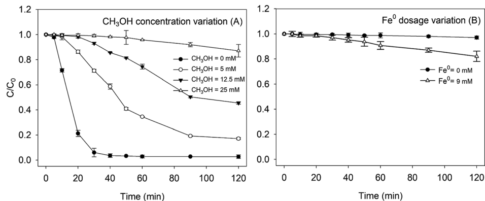
Fig. 3 Effect of methyl alcohol on the removal of RhB by the Fenton-like system [(A) pH = 4.0, [RhB] = 0.1 mM, [Fe 0 ] = 9 mM, [H 2 O 2 ] = 8 mM, and T = 25\text{ }^{\circ}\text{C} ; (B) pH = 4.0, [RhB] = 0.1 mM, [H 2 O 2 ] = 8 mM, and T = 25\text{ }^{\circ}\text{C} ].
