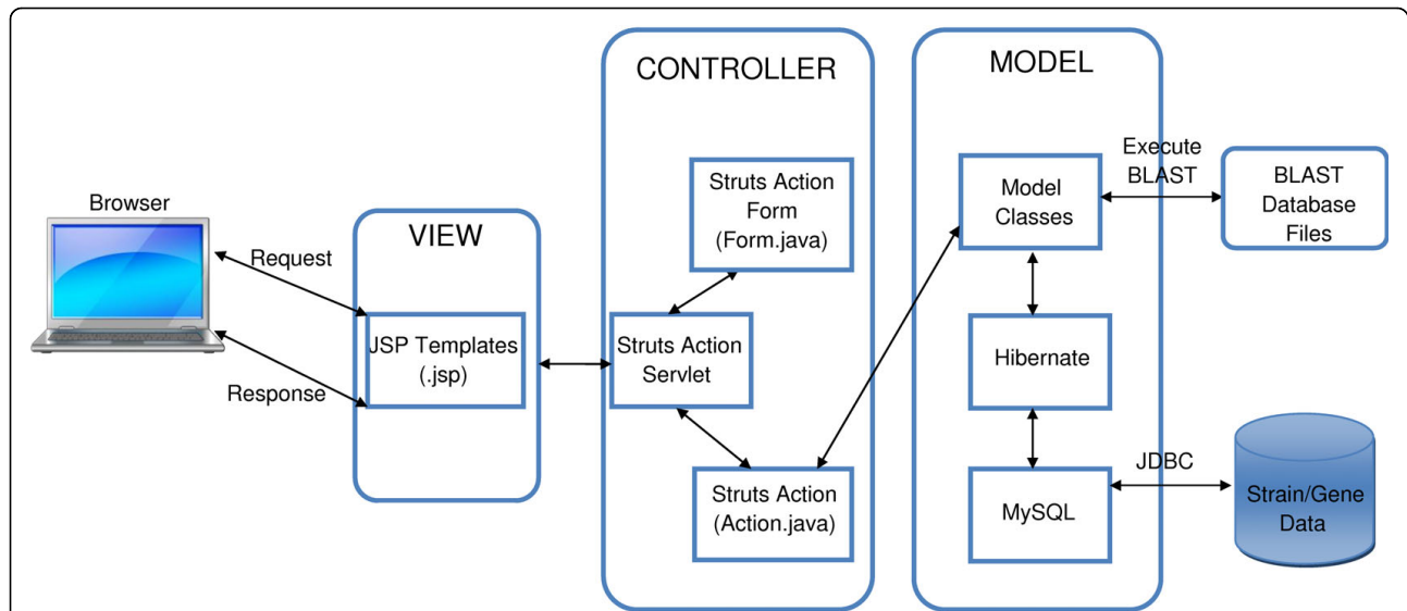
Figure 2 DraGnET software architecture. The DraGnET web application uses Struts to implement the Model-View-Controller (MVC) architecture. The view represents the presentation of the application and is implemented through Java Server Pages (JSP). The Controller is responsible for intercepting and translating user input into actions to be performed by the Model. The Controller receives the request from the browser, invokes a business operation and coordinates the view to be returned to the browser. The Struts Action servlet populates information from the JSP to the appropriate Struts Action Form then throws control to the Struts Action. The Struts Action gets data from the appropriate Struts Action Form and sends the information to the Model where certain actions like retrievals and updates will be performed. The Model is where communication with the database takes place through Hibernate. Hibernate is used to map Model Classes (Java objects) to tables in the database. Model Classes are also used to execute BLAST functionalities provided through the application's web interface. The Model represents enterprise data and the business rules that govern access to and updates of this data.
