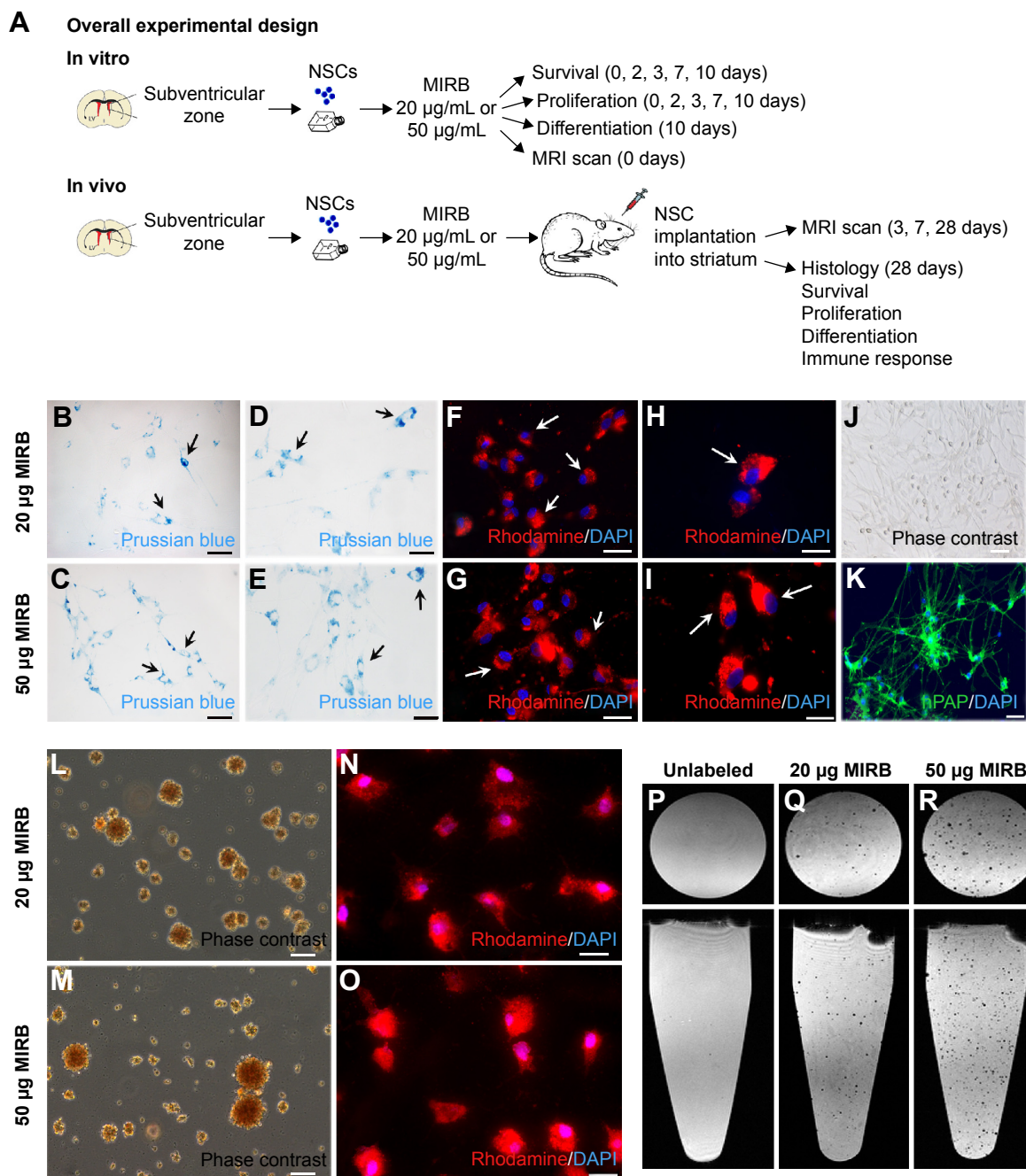
Figure 1 In vitro MIRB labeling and MRI imaging.
