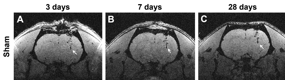
Figure S2 MRI of sham animals.
