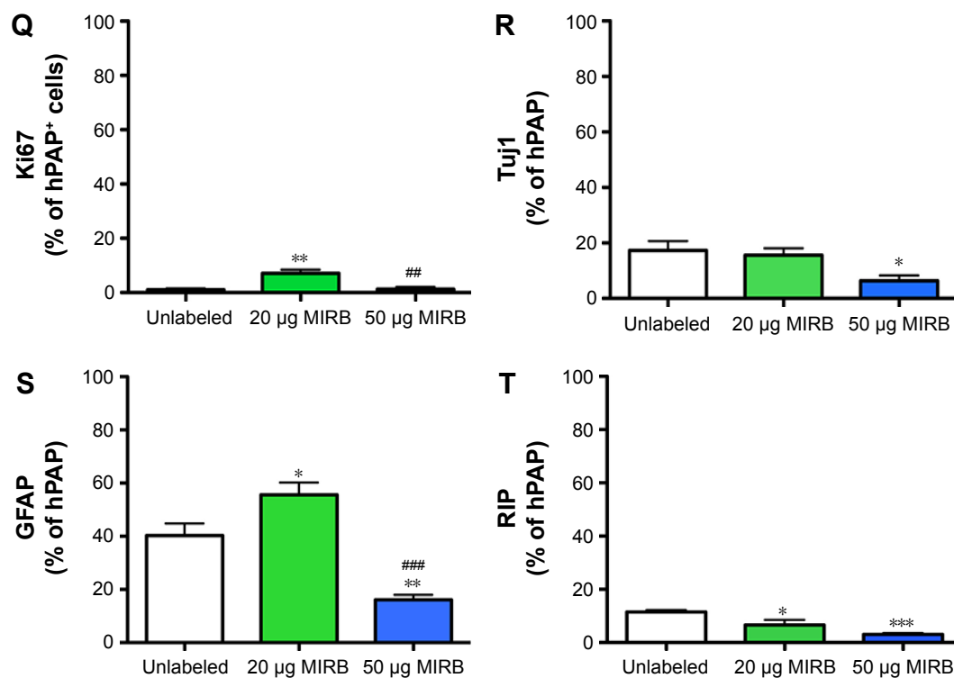
Figure 5 The proliferation and differentiation of transplanted NSCs are altered by MIRB labeling.
