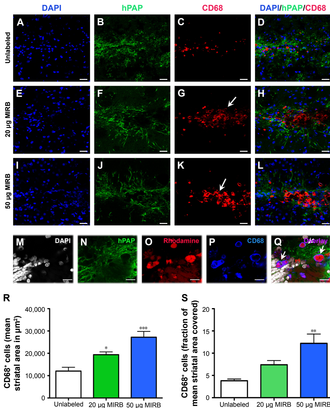
Figure 6 Transplantation of MIRB-labeled NSCs induces increased microglial activation and ectopic labeling of CD68 microglia.
