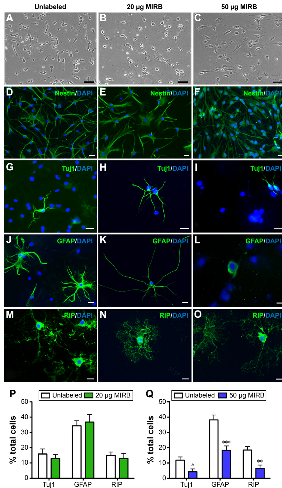
Figure 3 NSC differentiation rate and morphology are altered by MIRB labeling.
