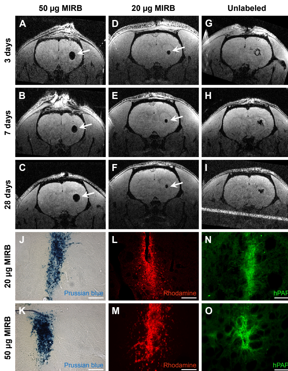
Figure 4 Extended in vivo tracking of MIRB-labeled NSCs.
