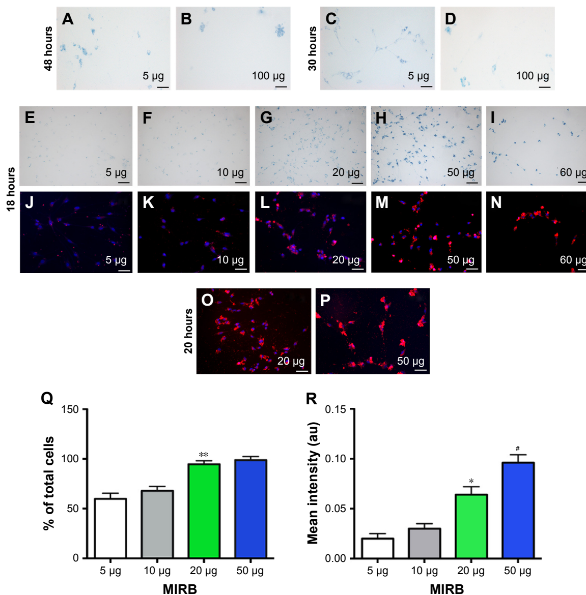
Figure S1 Optimization of MIRB dose.
