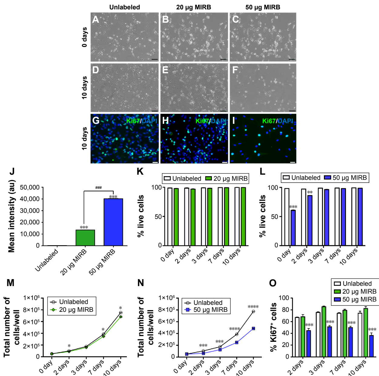
Figure 2 MIRB labeling affects NSC viability and proliferation.
