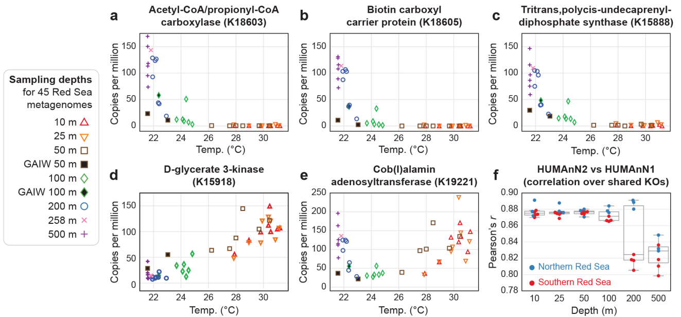
Figure 3: Thermocline-associated microbial enzymes in the marine pelagic zone.
