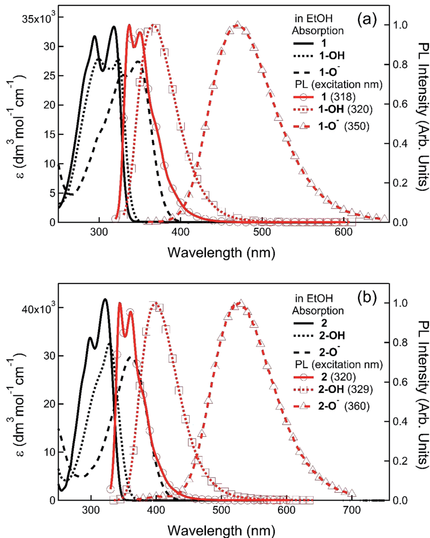
Fig. 2 The solution UV-visible absorption and photoluminescence spectra of the arylboronate esters ( 1 and 2 ), phenols ( 1-OH and 2-OH ) and phenoxides ( 1-O - and 2-O - ). 1-O - and 2-O - were obtained by mixing 1-OH ( 3.4 \times 10^{-5} M) or 2-OH ( 2.4 \times 10^{-5} M) with (n\text{-Bu})_4\text{NOH} ( 7.3 \times 10^{-4} M) in ethanol.
