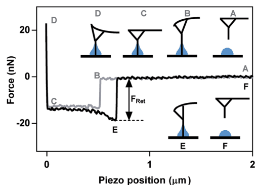
Fig. 1 Typical AFM force plot measurement depicts the series of events that occur during approach (grey) and retract (black) cycle of the AFM cantilever on the submicron-sized droplet. The retention force ( F_{\text{Ret}} ) is used to quantify the surface tension.
