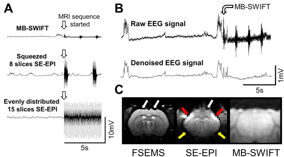
Fig. 6. Examples of the fMRI gradient switching artefacts in EEG signals (A), raw and denoised EEG signals obtained during EEG/MB-SWIFT fMRI (B), and EEG-electrode-induced image distortions (C) during simultaneous EEG-fMRI in an isoflurane-anesthetized rat. Panel A shows that the gradient artefacts are roughly 10 times higher during SE-EPI compared with MB-SWIFT (15 mV and 1.5 mV, respectively). The voltage scale is the same for all three EEG signals in section A, while a smaller voltage scale is used for the two signals in section B. The white arrows in panel C indicate the electrode-induced signal distortions in fast spin echo multi slice (FSEMS) and spin echo echo planar imaging (SE-EPI) images. Red arrows indicate signal pile-up artefacts in SE-EPI images. Yellow arrows show typical distortions in the lower brain regions around air cavities in SE-EPI fMRI images. Compared with FSEMS and SE-EPI images, no distortions were observed in MB-SWIFT images.
