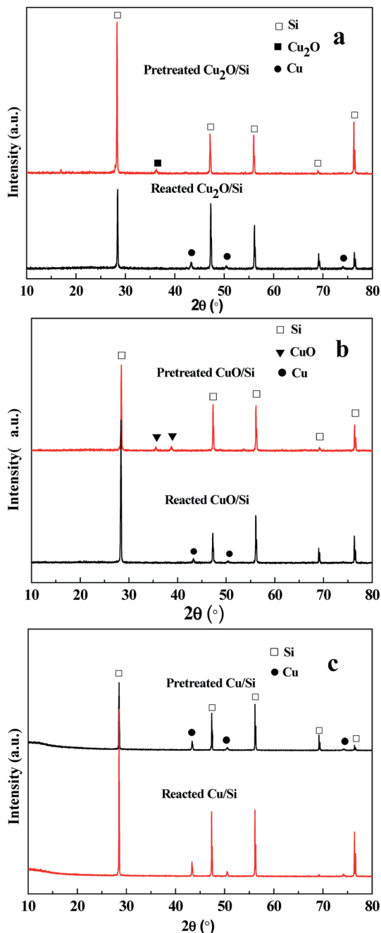
Fig. 5 XRD spectra of (a) \text{Cu}_2\text{O}/\text{Si} , (b) \text{CuO}/\text{Si} , and (c) \text{Cu}^0/\text{Si} mixtures after pretreatment and reaction. These mixtures were pretreated at 240\text{ }^\circ\text{C} for 2 h in a \text{N}_2 stream ( 20\text{ mL min}^{-1} ) and then reacted at 220, 240, and 260\text{ }^\circ\text{C} for 1 h, respectively. The reaction conditions: catalyst/Si, 40 g; weight ratios of \text{Cu}_2\text{O} , CuO, and \text{Cu}^0 to Si, 5 : 100, 5 : 100, and 8 : 100; methanol flow rate, 6\text{ mL h}^{-1} .
