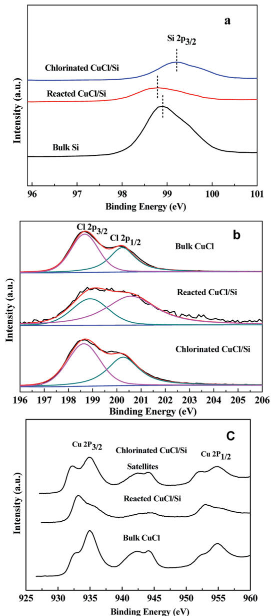
Fig. 3 XPS of Si 2p, Cl 2p, and Cu 2p of the bulk Si, bulk CuCl, reacted CuCl/Si, and chlorinated CuCl/Si samples. Reaction conditions: CuCl/Si weight ratio of 8 : 100, 40 g; methanol flow rate, 6 mL h -1 . The mixture reacted at 240 °C for 12 h, denoted as reacted CuCl/Si. After reacting for 12 h, the mixture was chlorinated with HCl (40 mL min -1 ) at 280 °C for 1.5 h, denoted as chlorinated CuCl/Si.
