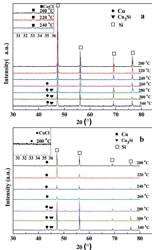
Fig. 1 XRD spectra of the CuCl/Si mixtures after pretreatment and reaction. (a) The CuCl/Si mixtures were pretreated at different temperatures of 200 – 340^\circ\text{C} for 2 h in a \text{N}_2 stream ( 20 \text{ mL min}^{-1} ). (b) After pretreating at a given temperature, the CuCl/Si mixtures reacted with methanol at 220 , 240 , and 260^\circ\text{C} for 1 h, respectively. The reaction conditions: CuCl/Si mixture, 40 g; CuCl/Si weight ratio, 8 : 100; methanol flow rate, 6 \text{ mL h}^{-1} . The insets are the amplified XRD peaks of CuCl phase.
