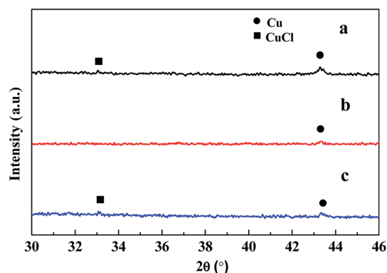
Fig. 2 XRD spectra of the CuCl/Si mixtures under different reaction conditions. (a) The CuCl/Si mixture was pretreated at 200^\circ\text{C} for 2 h in a \text{N}_2 stream ( 20 \text{ mL min}^{-1} ) and then reacted with methanol at 220 , 240 , and 260^\circ\text{C} for 1 h, respectively. (b) The CuCl/Si mixture reacted with methanol at 240^\circ\text{C} for 12 h. (c) After reacting for 12 h, the spent CuCl/Si mixture was chlorinated with \text{HCl} ( 40 \text{ mL min}^{-1} ) at 280^\circ\text{C} for 1.5 h. Reaction conditions: CuCl/Si weight ratio of 8 : 100, 40 g; methanol flow rate, 6 \text{ mL h}^{-1} .
