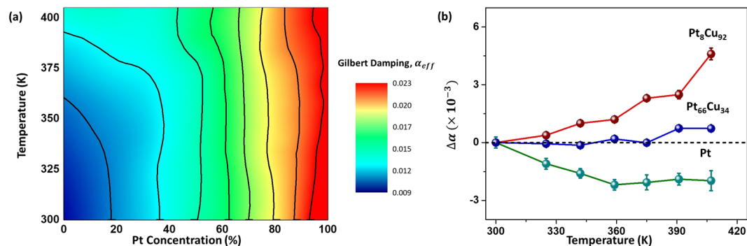
Figure 3. (a) Contour plot of \alpha for \text{Pt}_x\text{Cu}_{1-x} (5 nm)/Co(5 nm)/Ta(5 nm) trilayer device with temperature for varying Pt concentrations. (b) \Delta\alpha of \text{Pt}_x\text{Cu}_{1-x} (5 nm)/Co(5 nm)/Ta(5 nm) for x = 8\% , 66\% and 100\% .
