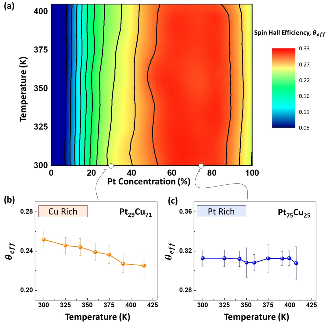
Figure 4. (a) Contour plot of \theta_{eff} for Pt_xCu_{1-x} (5 nm)/Co(5 nm)/Ta(5 nm) trilayer device with temperature for varying Pt concentrations. (b) and (c) Temperature dependence of \theta_{eff} for Cu-rich and Pt-rich Pt_xCu_{1-x} (5 nm)/Co(5 nm)/Ta(5 nm) trilayer device with x = 29\% and 75\% respectively.
