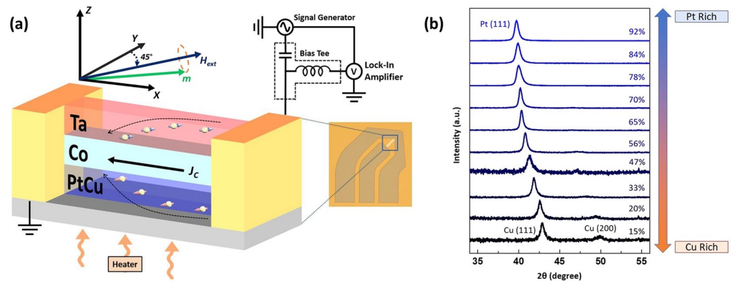
Figure 1. (a) Schematic illustration of high temperature ST-FMR setup. Optical image of the device is as shown in the inset. (b) X-ray diffraction pattern of 80 nm thick \text{Pt}_x\text{Cu}_{1-x} samples showing the shift between the Pt(111) to the Cu(111) peak.
