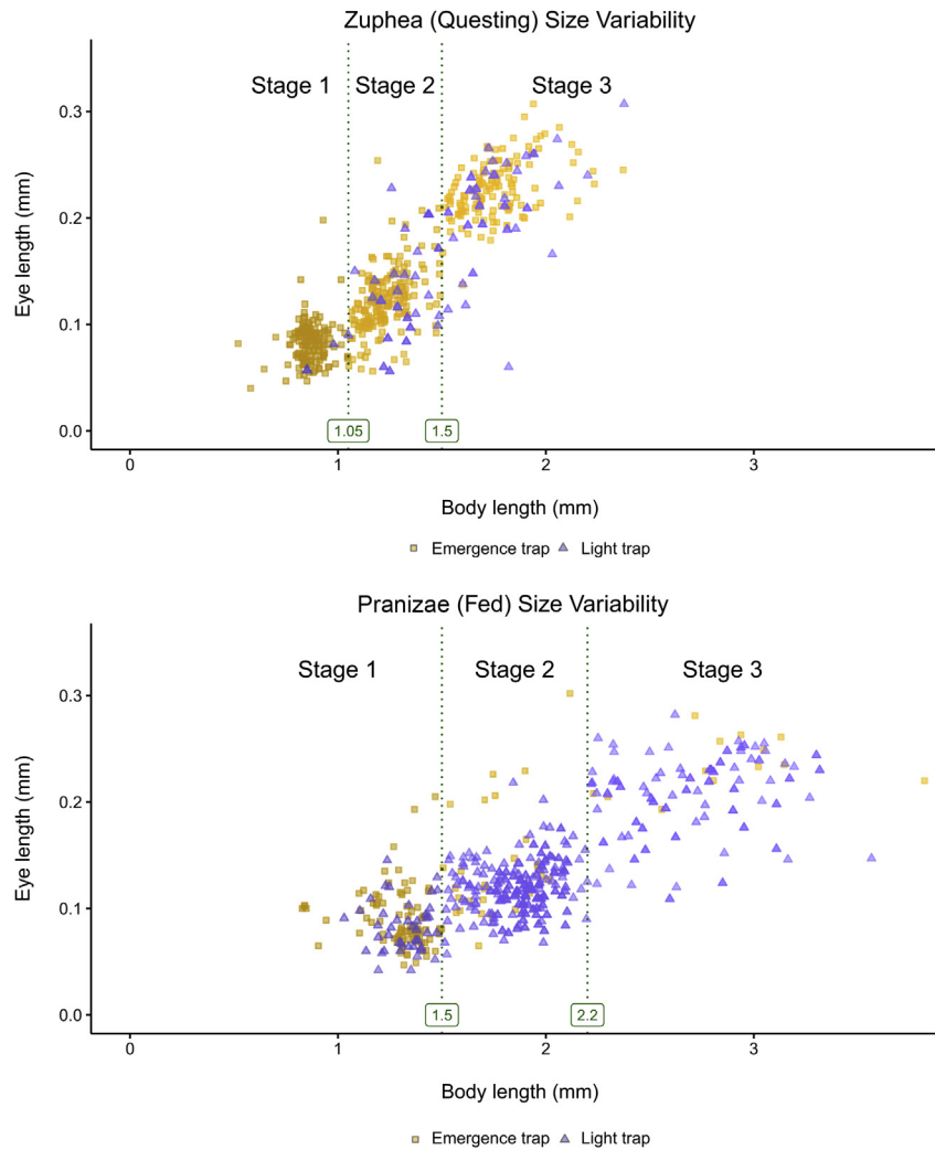
Fig. 3. Scatterplots of total body length in mm plotted against eye length in mm along the long axis. The upper plot shows measurements for Zuphea and the lower plot for Pranizae . The body length cutoff values separating juvenile stages are shown as a dotted-green line. Gnathiids collected from emergence traps are seen as gold-filled squares and those collected from light traps are presented as purple-filled triangles. Differences in the ontological sampling bias of these two trap designs can be seen by comparing the two scatterplots. (For interpretation of the references to colour in this figure legend, the reader is referred to the web version of this article.)
