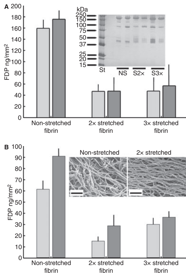
Fig. 4. Release of soluble fibrin degradation products (FDP) from the surface of clots. (A) Fibrin containing 200 \text{ nmol L}^{-1} plasminogen was prepared as in Fig. 3 and fibrinolysis was initiated with 15 \text{ nmol L}^{-1} tissue-type plasminogen activator (tPA). (B) Plasminogen-free fibrin was prepared as in Fig. 2 and fibrinolysis was initiated with 1 \mu\text{mol L}^{-1} plasmin. At 15-min intervals the fluid surrounding the fibrin was withdrawn and its ethanol-soluble FDP content was measured as described in Methods. The amount of released FDP is shown (normalized for unit surface area of the fibrin clots) for the 1 st (light gray bars) and 3 rd (dark gray bars) 15-min period of the lysis. Data are presented as mean and SD ( n = 4 ) and the differences between the non-stretched and stretched fibrins are significant at the P < 0.01 level according to the Kolmogorov-Smirnov test. (Inset A) After adjustment for protein concentration the samples in (A) were subjected to SDS electrophoresis on 12.5% polyacrylamide gel under non-reducing conditions and silver-stained. (Inset B) After withdrawal of the fluid phase after 45-min digestion the samples in B were fixed in glutaraldehyde and SEM images were taken as described in Methods; truncated fibers are indicated by white arrows, scale bar = 2 \mu\text{m} .
