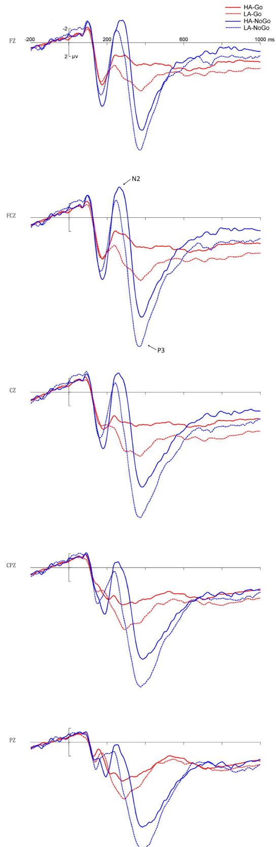
Figure 1. Grand average of ERP. The grand average of ERP elicited in the low-altitude group (LA, dotted lines) and the high-altitude group (HA, solid lines) at the central sites (Fz, FCz, Cz, CPz, Pz) in the Go (Go, red lines) and NoGo (NoGo, blue lines) conditions.
