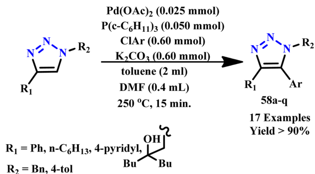
Scheme 47 Microwave-assisted Pd catalyzed arylation of 1,4-disubstituted 1,2,3-triazole derivatives ( 58a–q ). 90
