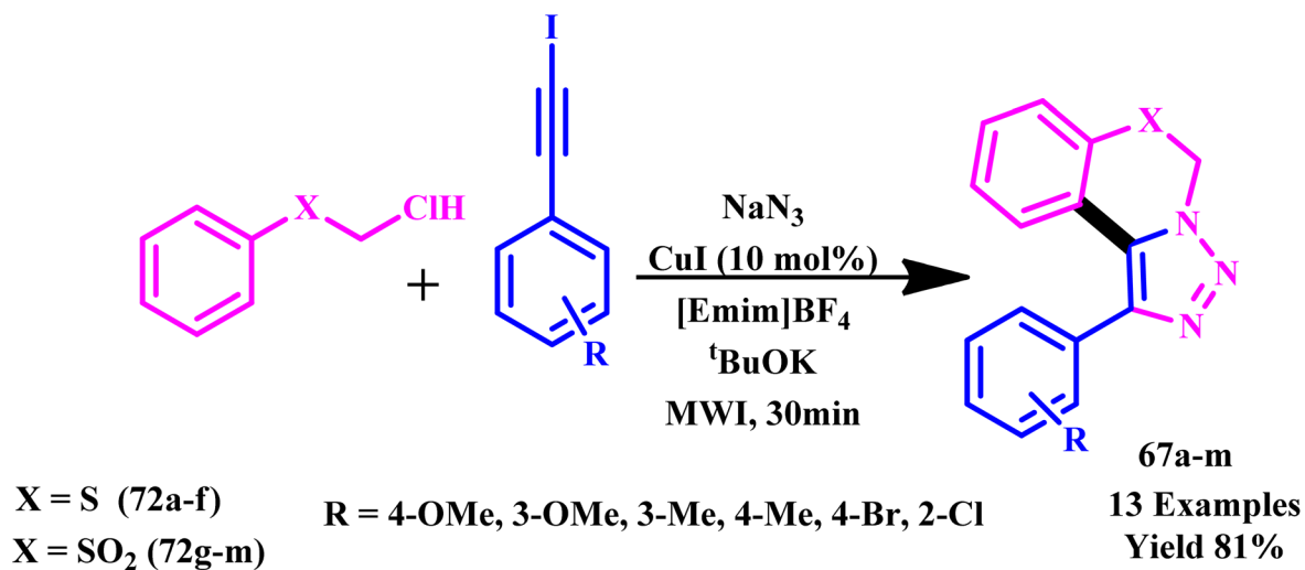
Scheme 56 Microwave-assisted synthetic route for fused benzo[e]1,2,3-triazoles (67a–m). 103
