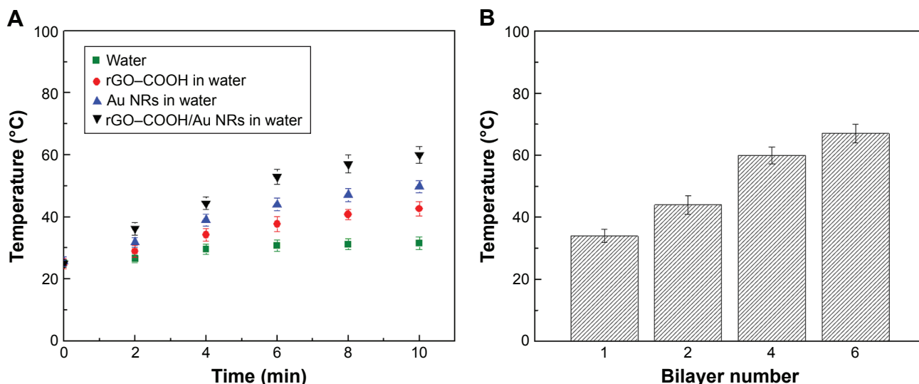
Figure 3 (A) Change in temperature of rGO-COOH, Au NRs, and (rGO-COOH/Au NRs), in water after NIR radiation (808 nm, 0.7 W cm -2 ). Pure water was irradiated similarly as a control. (B) The temperature changes of the rGO-COOH/Au NRs multilayer are profiled over layer number after 10 minutes radiation.
