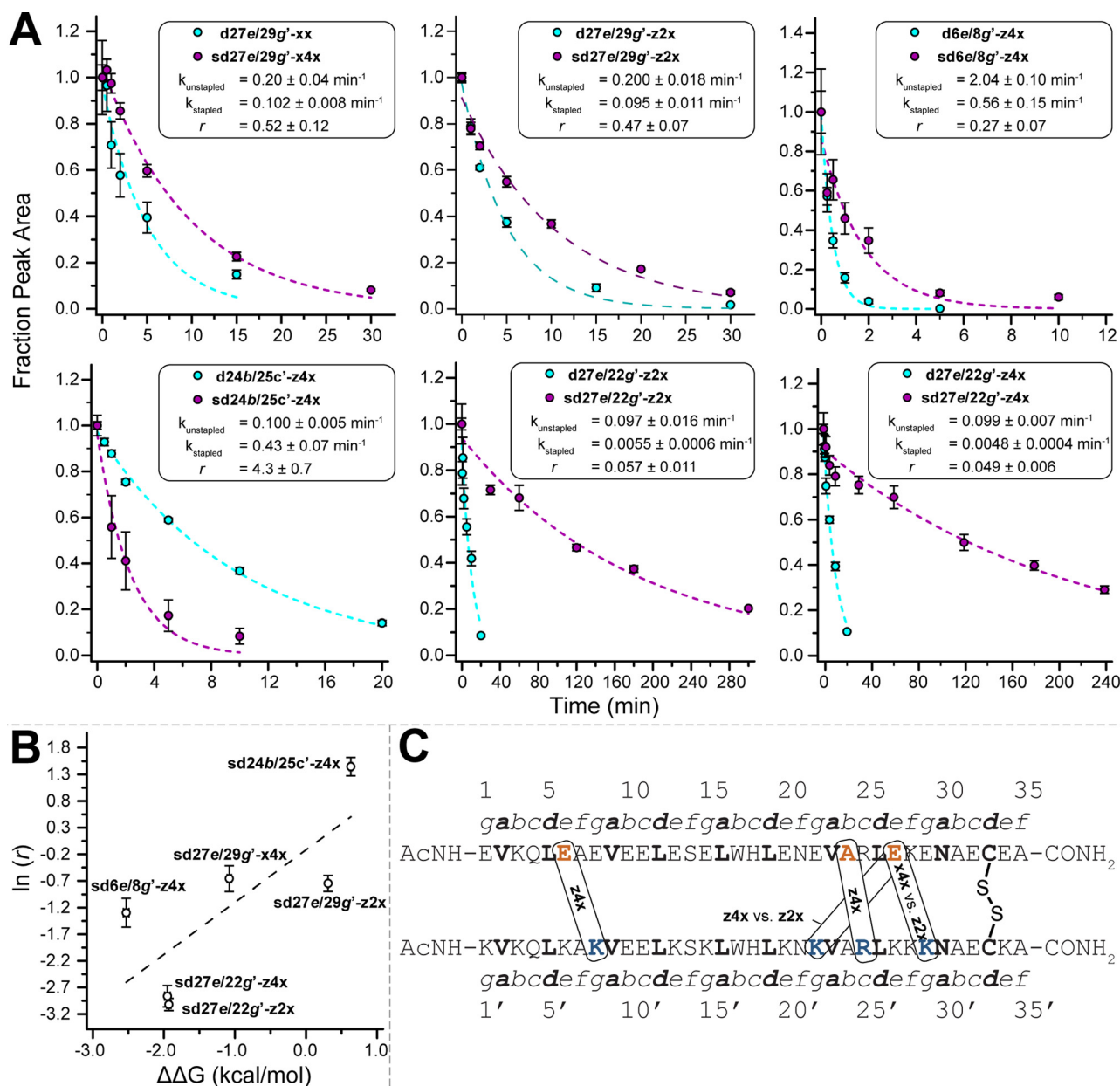
Fig. 3 (A) Proteolysis of selected unstapled and stapled variants by proteinase K (17 \mu\text{g mL}^{-1} ) at 15 \mu\text{M} protein concentration in 20 mM sodium phosphate buffer (pH 7) as monitored by HPLC. Data points represent the average of three replicate experiments for unstapled variants (cyan) and for stapled variants (magenta). Coloured dotted lines represent fits of the data for each variant to a mono-exponential decay function, which was used to determine apparent proteolysis rate constants k and rate constant ratios r . (B) The impact of PEG-stapling on the conformational stability of these variants ( \Delta\Delta G ) plotted against the natural logarithm of r . Black dotted line represents fit of the \ln(r) vs. \Delta\Delta G data to a linear equation. Slope = 0.98 \pm 0.40 ; R^2 = 0.60 . (C) Location and identity of the staples investigated here within the disulfide-bound coiled coil.
