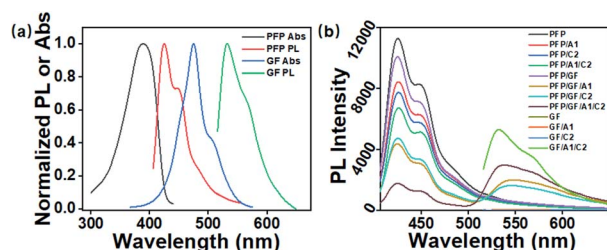
Fig. 1 (a) Absorption spectra and fluorescence spectra of PFP and geniferdine (GF). (b) The FRET between PFP and GF/DNA. The concentrations of PFP, DNA, and GF were 20 \mu\text{M} , 1 \mu\text{M} , and 5 \times , respectively. Systems containing PFP were irradiated at 380 nm. Direct excitation of GF/DNA at 490 nm without PFP is also listed.
