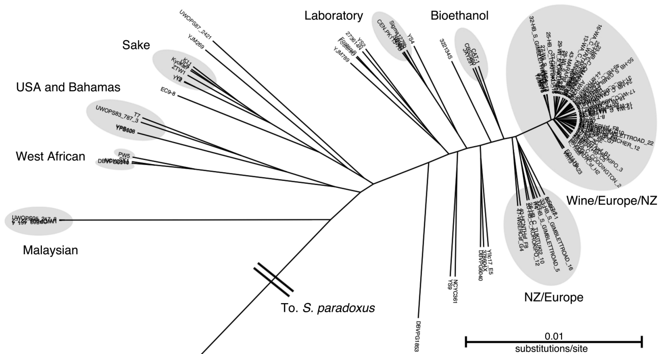
Figure 1. Rooted phylogeny of 112 S. cerevisiae strains created using the 106 loci dataset with S. paradoxus as the outgroup reconstructed using the Bayesian methods implemented in BEAST (v1.7.5; Drummond and Rambaut 2007). The NZ strains cluster and interdigitate with the wine/European group.
