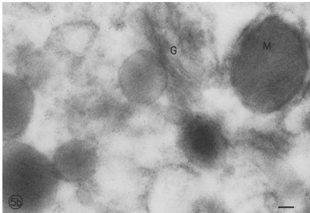
FIGURE 5 Electron micrographs of ultrathin frozen sections of adult chicken pancreas, stained with antilectin gamma globulin followed by ferritin-labeled goat anti-rabbit IgG. Extracellular space between acinar cells (bracket) shows heavy labeling (Fig. 5 a ). Relatively sparse intracellular labeling (Fig. 5 b ). M , mitochondrion; G , Golgi apparatus. Calibration bar, 0.1 \mu m.
