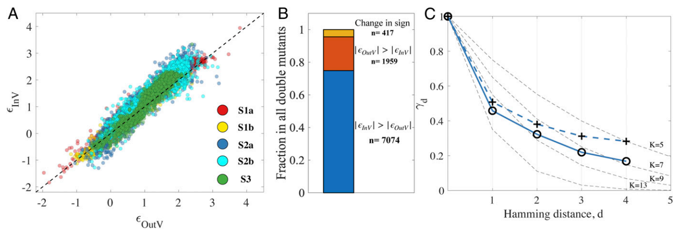
Fig. 6. Effect of encapsulation on epistasis and ruggedness of the fitness landscape. (A) \epsilon in the encapsulated (y-axis, \epsilon_{InV} ) versus the nonencapsulated (x-axis, \epsilon_{OutV} ) condition for all double mutants in the central 21-nt region (i.e., 1,890 double mutants), for each of the five ribozyme families as indicated by color. The families are plotted separately in SI Appendix, Fig. S11 . The dotted black line indicates the identity line. High correlations are observed, but \epsilon_{InV} magnitudes tend to be higher than \epsilon_{OutV} magnitudes ( SI Appendix, Table S3 ). (B) Bar chart showing the total fraction of double mutants exhibiting |\epsilon_{InV}| > |\epsilon_{OutV}| (blue) or |\epsilon_{OutV}| > |\epsilon_{InV}| (red) when \epsilon_{OutV} and \epsilon_{InV} have the same sign, and the fraction for which \epsilon_{OutV} and \epsilon_{InV} have opposite sign (yellow). The total number of sequences ( n ) within each group is indicated. The predominance of |\epsilon_{InV}| > |\epsilon_{OutV}| indicates greater epistasis when encapsulated. (C) Ruggedness (epistatic correlation \gamma_d ) of the fitness landscape as a function of hamming distance d for family S2a, illustrating lower correlation in the encapsulated (open circles) versus nonencapsulated (crosses) condition. The gray dashed lines depict the theoretical \gamma_d dependence for the NK model landscape with N = 21 and K as labeled in the plot.
