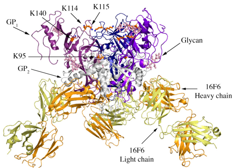
Figure 1. Cartoon representation of trimer of SUDV-Bon GP 1,2 bound to 16F6. The GP 1 chains are colored in various shades of blue and GP 2 chains are colored in white. The light chain of 16F6 is shown in pale yellow and the heavy chain of 16F6 is colored bright orange. The sugar residues on the glycoprotein are shown in ball and colored cyan. Lysine residues critical for receptor binding are shown in ball and stick and colored orange.
