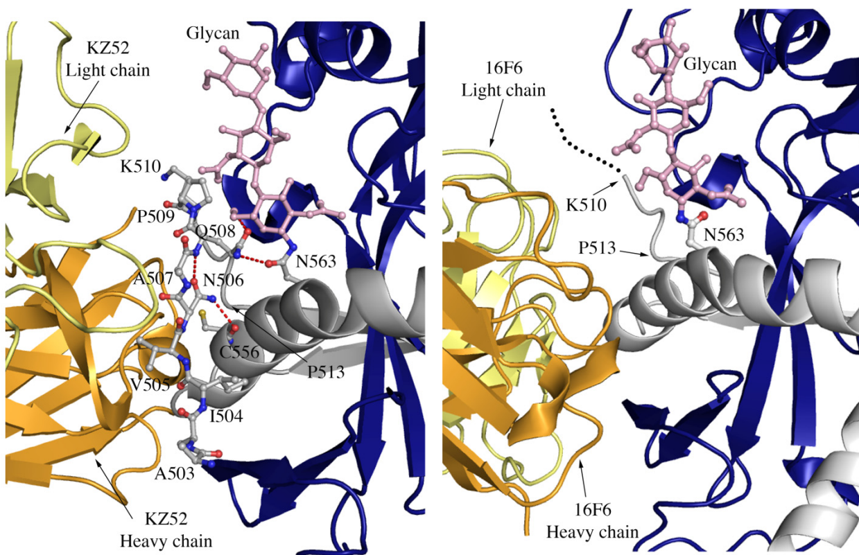
(A) EBOV GP 2 - N terminal peptide
