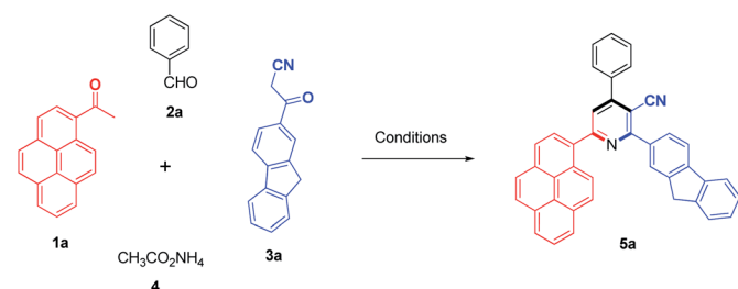
Scheme 1 Model reaction.
