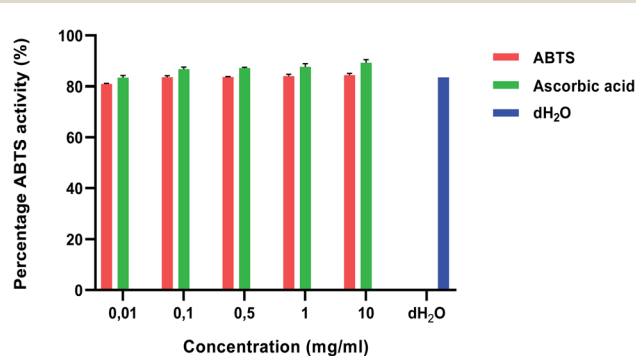
Fig. 2 ABTS scavenging activities of Tulbaghia violacea water extracts. Values are expressed as mean ± SD ( n = 3 ). Ascorbic acid and distilled water was used as a standard and control, respectively.
