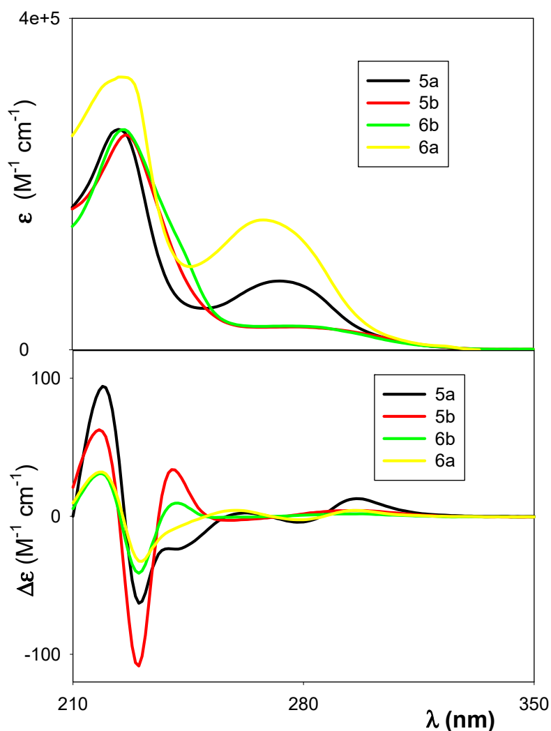
Figure 2. UV (top) and circular dichroism (CD) (bottom) spectra of macrocycles 5 and 6 . Concentrations: 10^{-5} \text{ M} for UV and 2.2\text{--}2.6 \times 10^{-6} \text{ M} for CD spectroscopy in MeCN.
