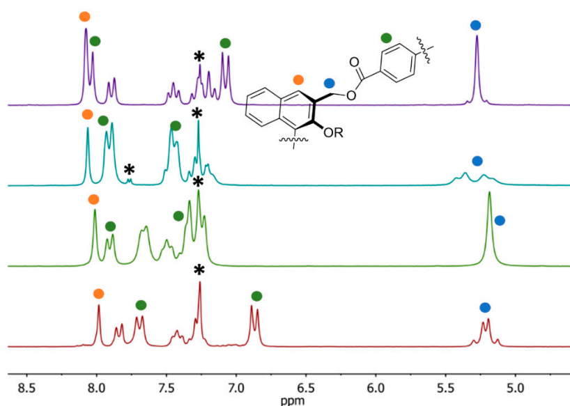
Figure 1. Aromatic and \text{CH}_2 benzylic ester region for the ^1\text{H} NMR spectra ( \text{CDCl}_3 , 200 MHz, 25 °C) of macrocycles (from top to bottom) 5a , 5b , 6b , 6a . The asterisk marks impurities and residual solvent.
