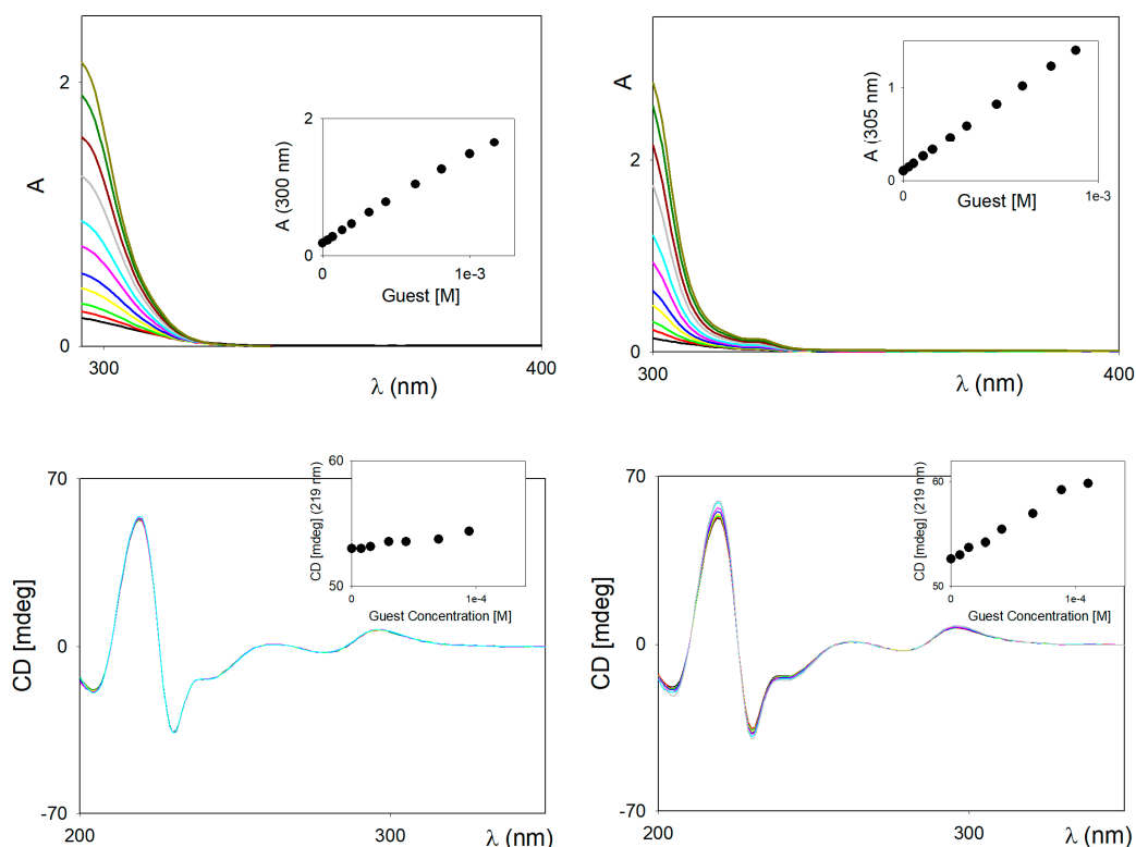
Figure 3. UV (top) and CD (bottom) titration of macrocycle 5a and hydroquinone (left) and 1,4-dimethoxybenzene (right). Concentrations: 10^{-5} M for UV and 10^{-6} M for CD spectroscopy in MeCN.
