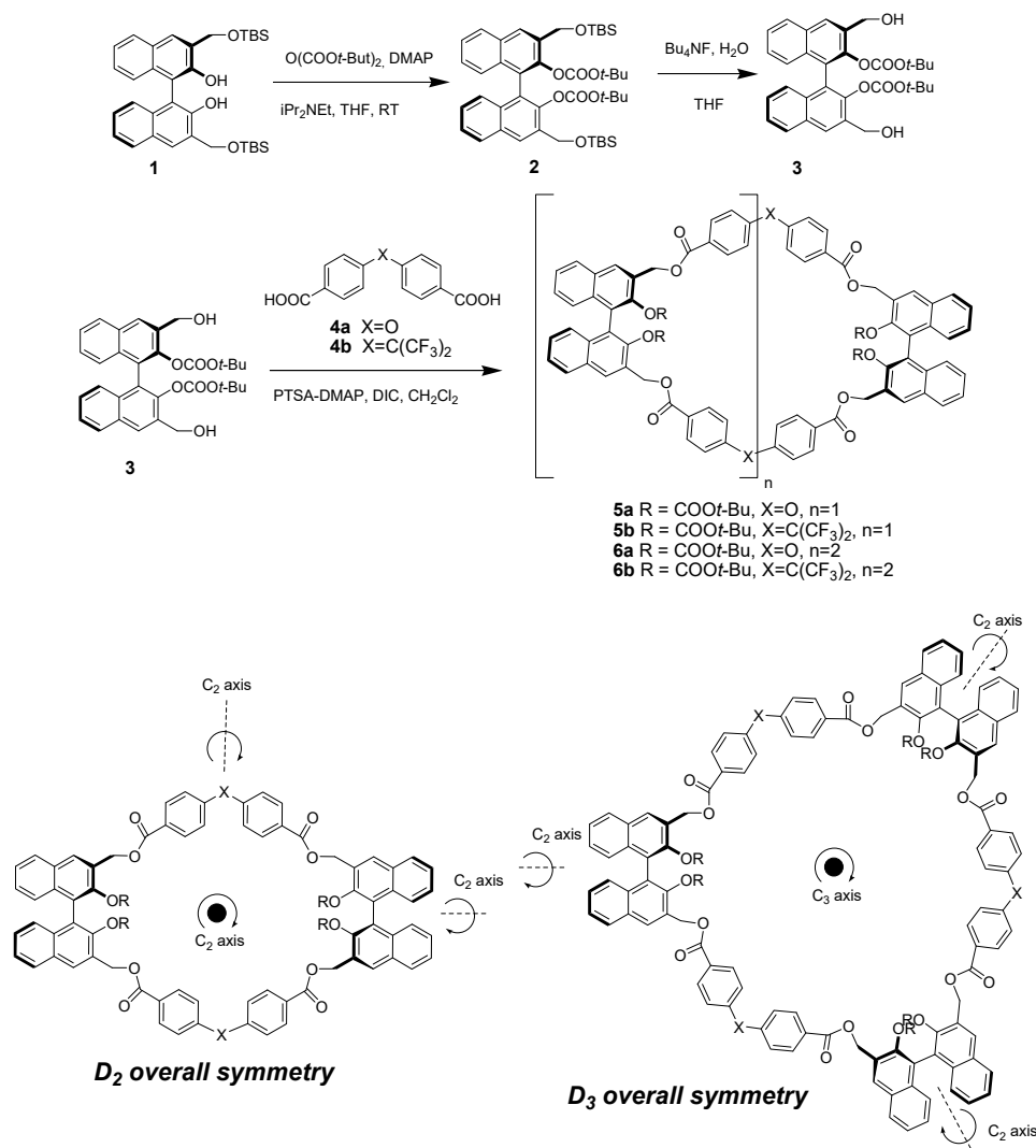
Scheme 1. Synthesis of suitable precursors and cyclization to form macrocycles 5 and 6.
