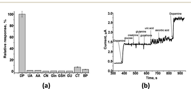
Fig. 5 Characterization of nAuCu/nAuPt/GCE sensor: selectivity (a) and possible interference effect (b) for different compounds without and with the addition of 0.2 mM dopamine (DA). Glucose (GU), creatinine (CN), glutamine (Gln), glutathione (GSH), uric acid (UA), ascorbic acid (AA), catechol (CT) and bisphenol (BP). The analytical signals under the working potential +200 mV are presented in relative units (%) related to the maximal current signal on DA (100%).
