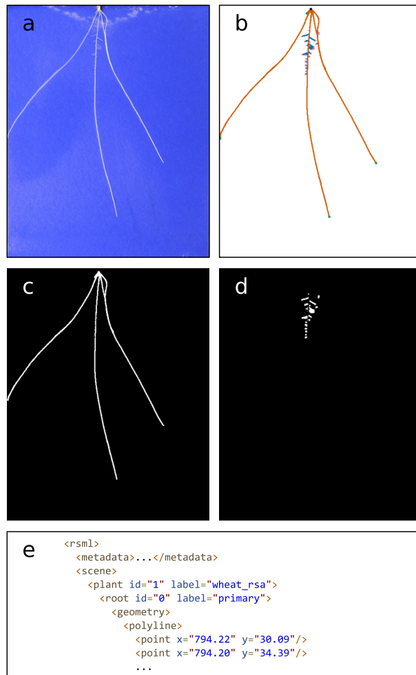
Figure 11: Example output from RootNav 2.0. (a) Input image. (b) Colour-coded segmentation mask. (c, d) Binary segmentation masks for first- and second-order roots. (e) A sample of the RSML file representing the entire architecture.
