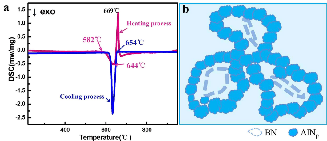
Figure 3. The formation of network structure in AlN p /Al composite. (a) DSC analysis of the 16.4% sample. (b) A network formation schematic: forming a closed and interconnected AlN p circle in spatial.
