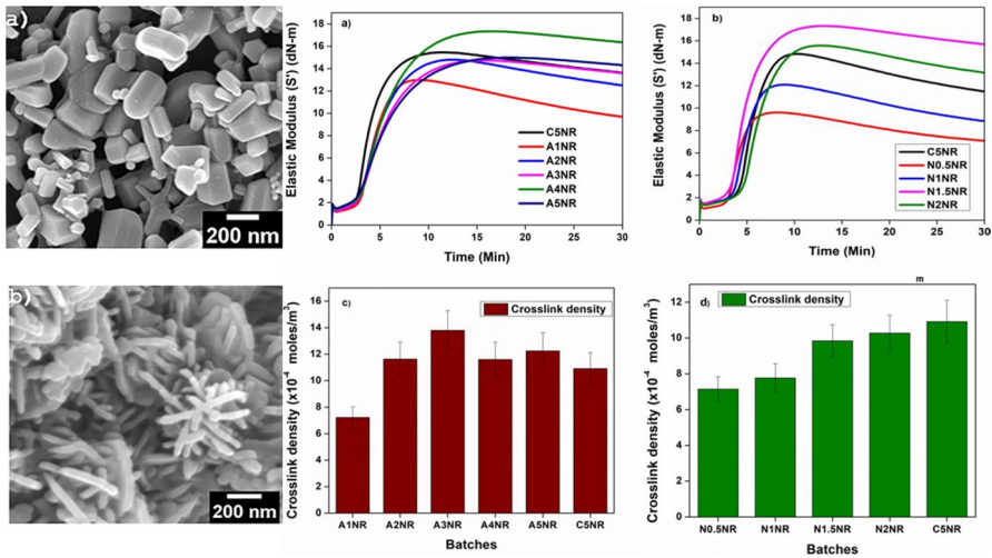
Fig. 10 a and b SEM images of conventional and active ZnO, Cure characteristics and Crosslink density of rubber composites [111]
